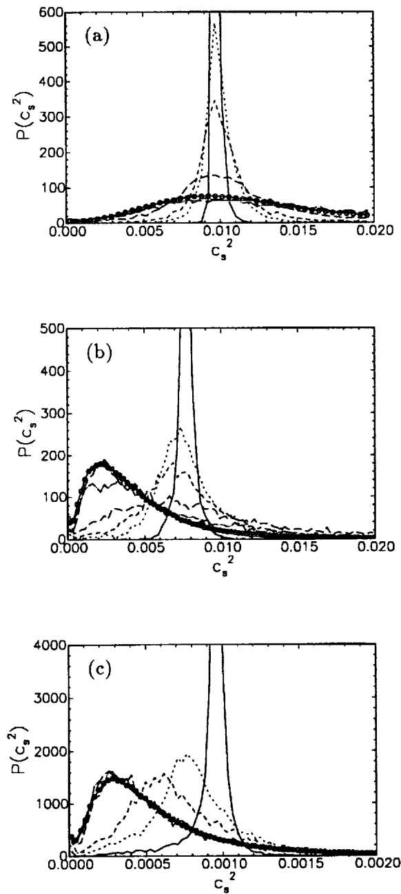
FIGURE 14. Probability-density functions of dynamic model coefficient c_s^2 for different time steps, n . — : n=2 ; ..... : n=10 ; - - - - : n=20 ; - · - · : n=80 ; - - - - : n=320 ; - - - - : n=640 ; o : n \sim 38,000 . Different graphs are at different heights above the wall: (a) is at y^+ = 641 , (b) at y^+ = 108 and (c) at y^+ = 12 .
