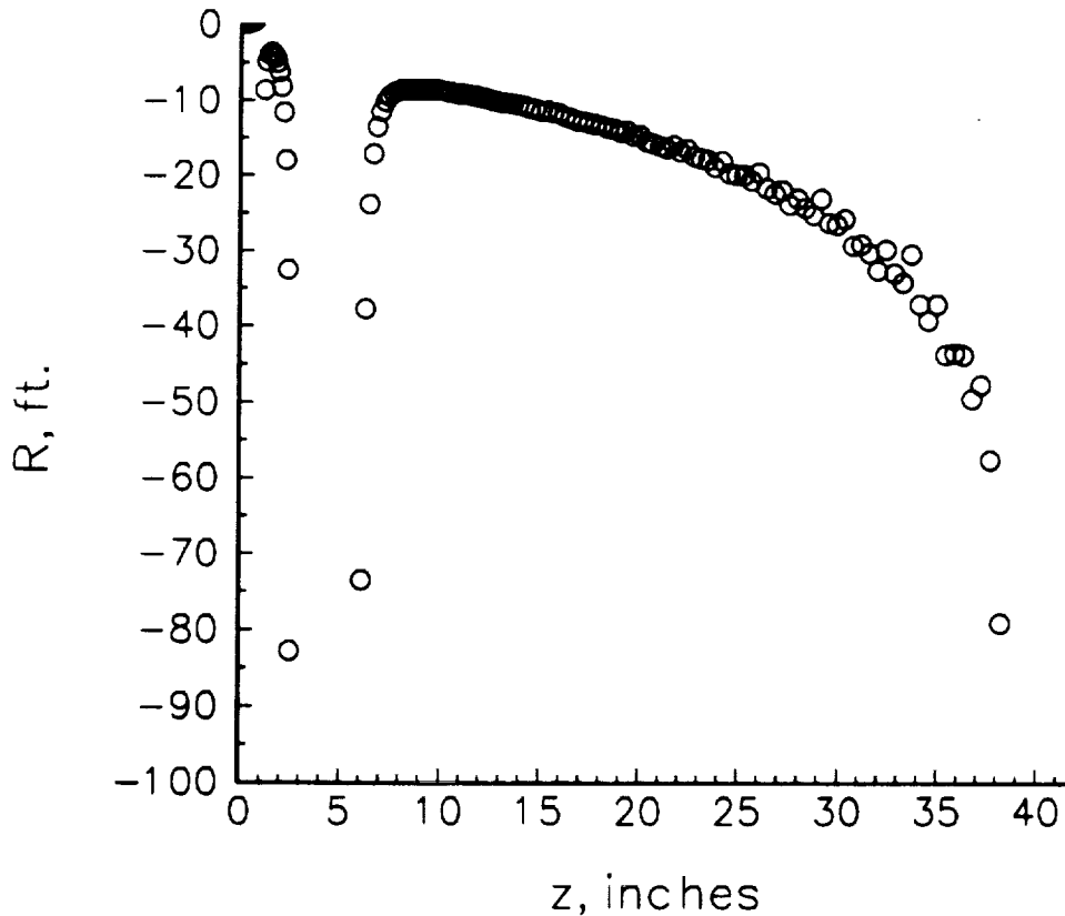
Figure 1: Radius of Curvature for Mach 6 Test Case
