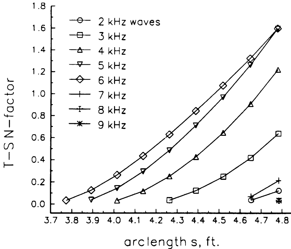
Figure 9: T-S N-Factors in Long Mach 2.4 Square Nozzle
