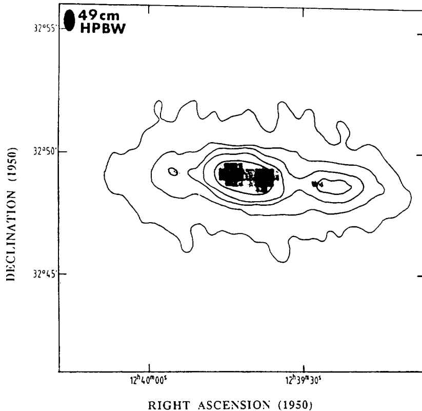
FIGURE 3 A greyscale image of the reconstructed 50\mu\text{m} image of the edge-on spiral NGC 4631 with contours of the 49cm non-thermal radio emission overlaid (Werner 1985). A distinct spatial correlation is evident between the features seen in both the radio and far-infrared.
