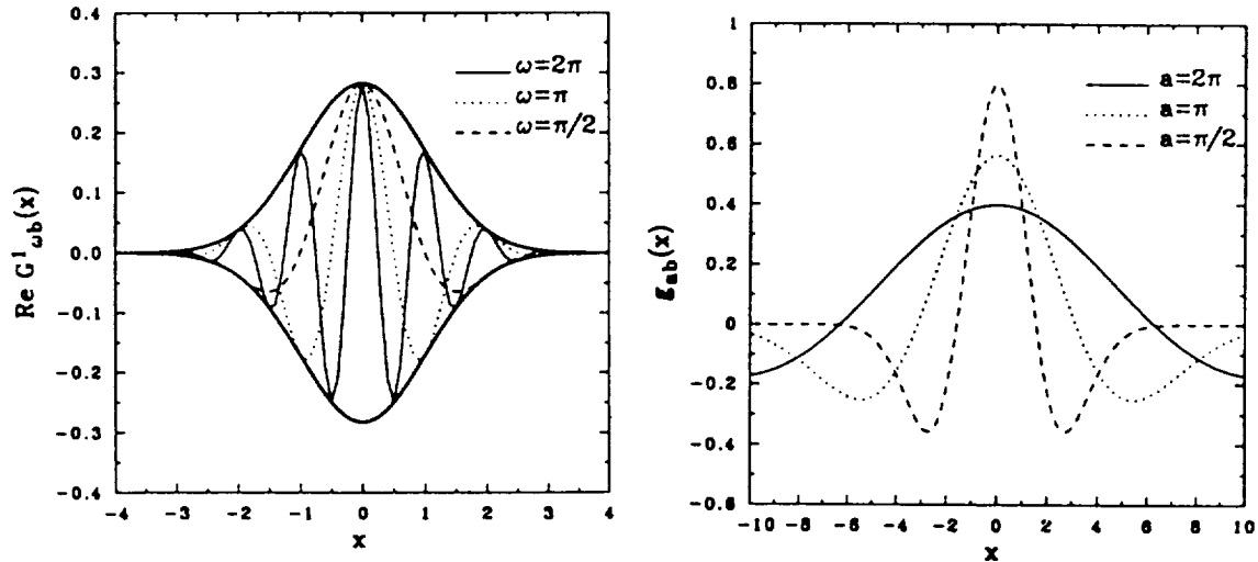
FIGURE 1 The functions g_{ab} and \text{Re } G^I_{\omega b} for three values of a and \omega ( b = 0 ). The Gabor transform has a fixed window size in contrast to the wavelet transform's flexible window (Martinez et al. 1993).
