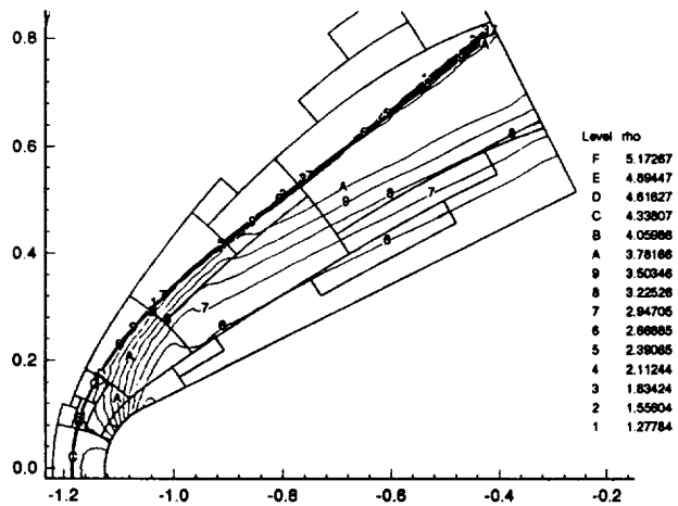
Figure 10. M = 5 flow over a 26.56° wedge with a blunt leading edge—contours of density.
