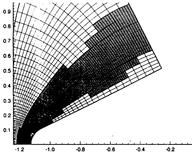
Figure 9. Grid system for a 26.56° wedge with a blunt leading edge—coarse grid is 32 × 48; 47.6% of the coarse grid cells are refined.
