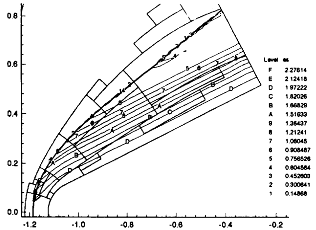
Figure 11. M = 5 flow over a 26.56° wedge with a blunt leading edge—contours of entropy.
