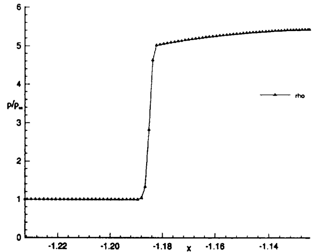
Figure 12. M = 5 flow over a 26.56° wedge with a blunt leading edge—plot of normalised density on the stagnation stream line versus axial location (leading edge is at x = -1.125 ; radius of curvature of leading edge is 0.125).
