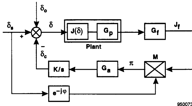
Figure 2. A single-dimensional extremum-searching algorithm.
