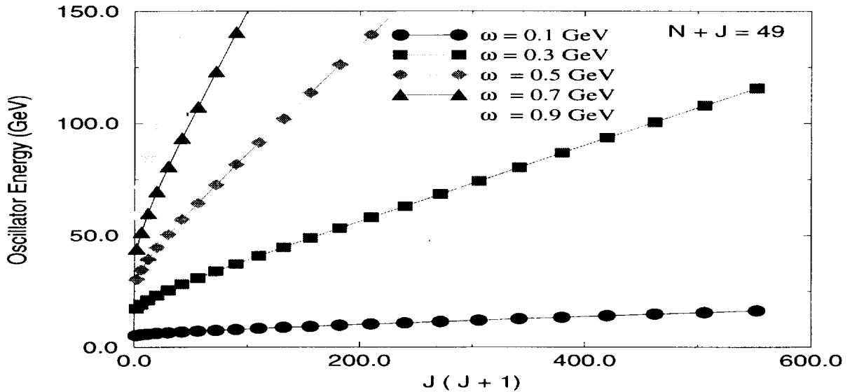
Figure 4: Energy levels of the N + J = 49 band as a function of J(J + 1) for different oscillator frequencies.
