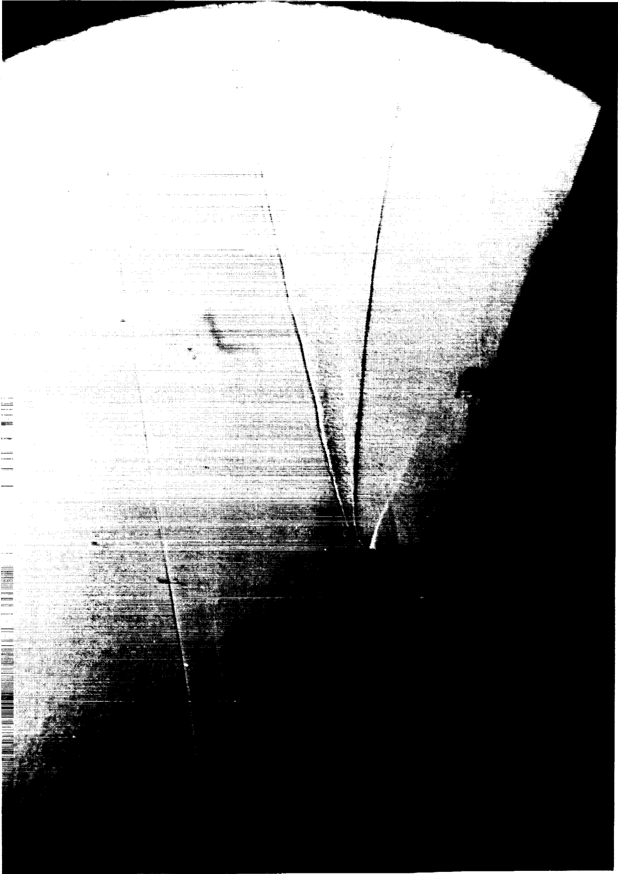
Figure 24. Shadowgraphs of jet plume, off-design test conditions. (a) P_{t_\infty} = 6895 \text{ kPa} , P_{t_j}/P_{t_\infty} = 79 , Run 24.
