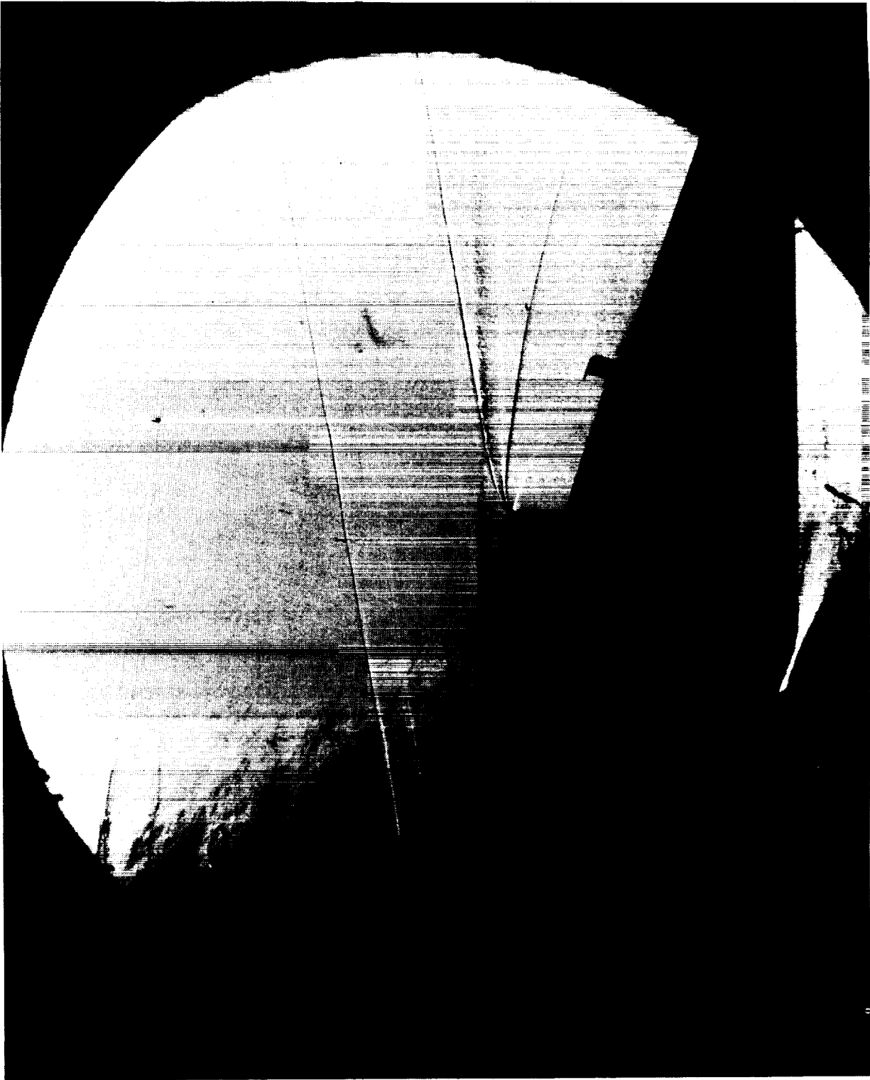
Figure 24. Continued. (d) P_{t_{\infty}} = 3447 kPa, P_{t_j} / p_{\infty} = 463 , Run 22.
