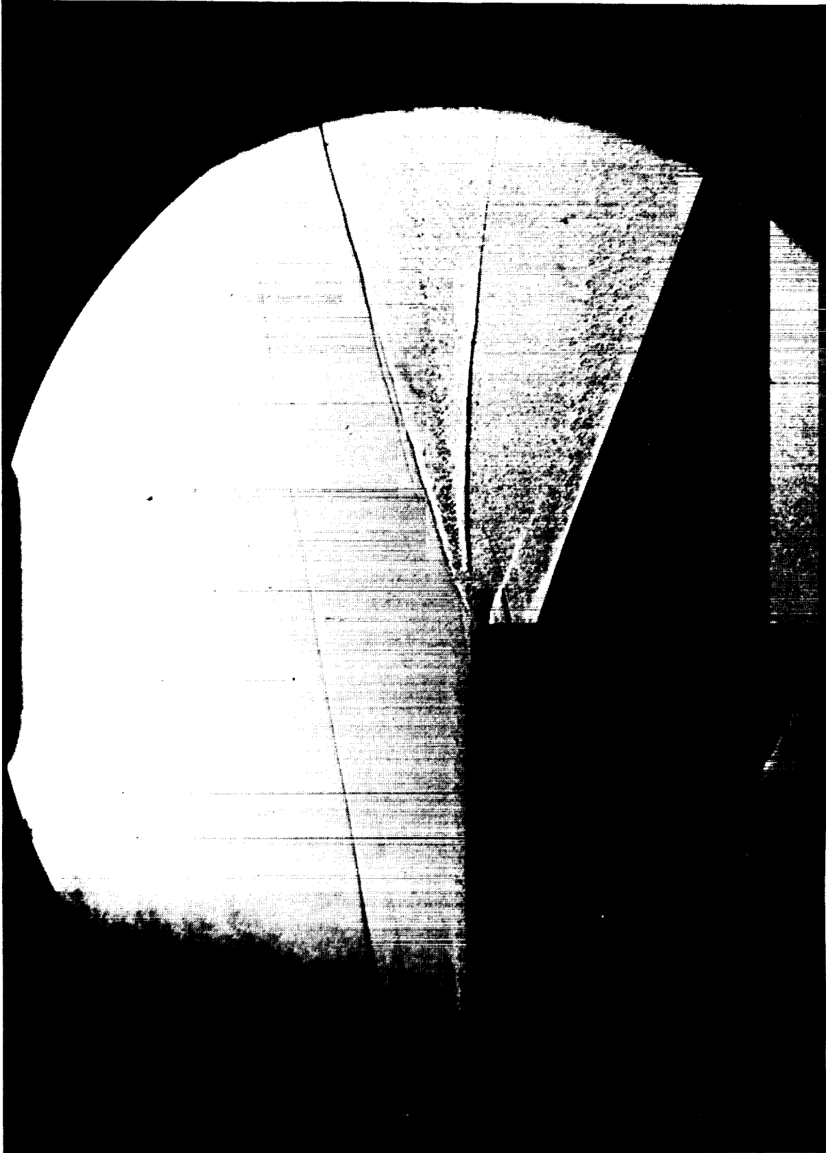
Figure 24. Concluded. (f) P_{1,\infty} = 3447 \text{ kPa} , P_{1j}/p_\infty = 620 , Run 11.
