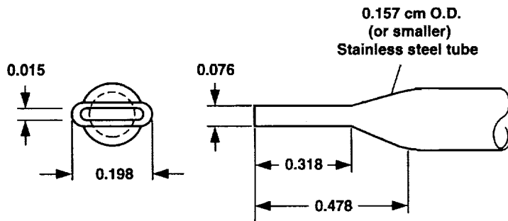
Detail of area "A" above
