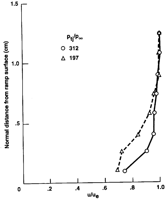
Figure 28. Boundary layer profiles from aft ramp rake.
