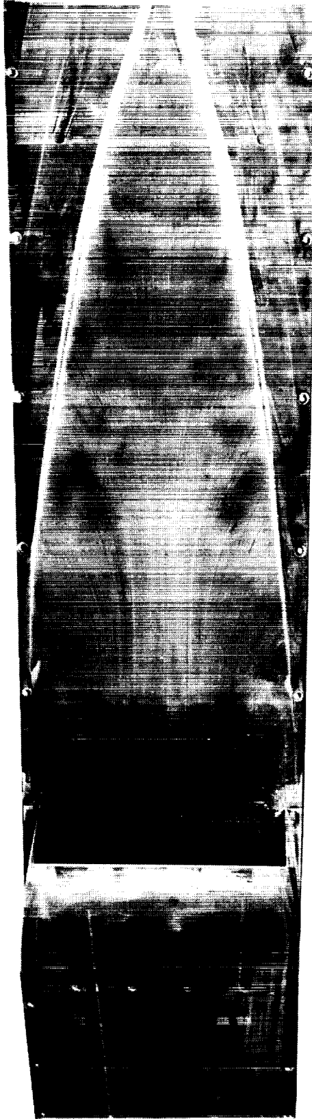
Figure 18. Oil flow photographs of model, baseline test conditions; P_{t_\infty} = 6895 \text{ kPa} , P_{t_1}/p_\infty = 310 , Run 8. (a) Ramp and cowl, top view.
