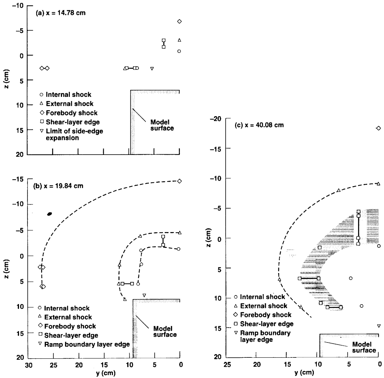
Figure 38. Shock-wave and shear-layer locations obtained from probe data, baseline test conditions. (a) x = 14.78 cm; (b) x = 19.84 cm; (c) x = 40.08 cm.
