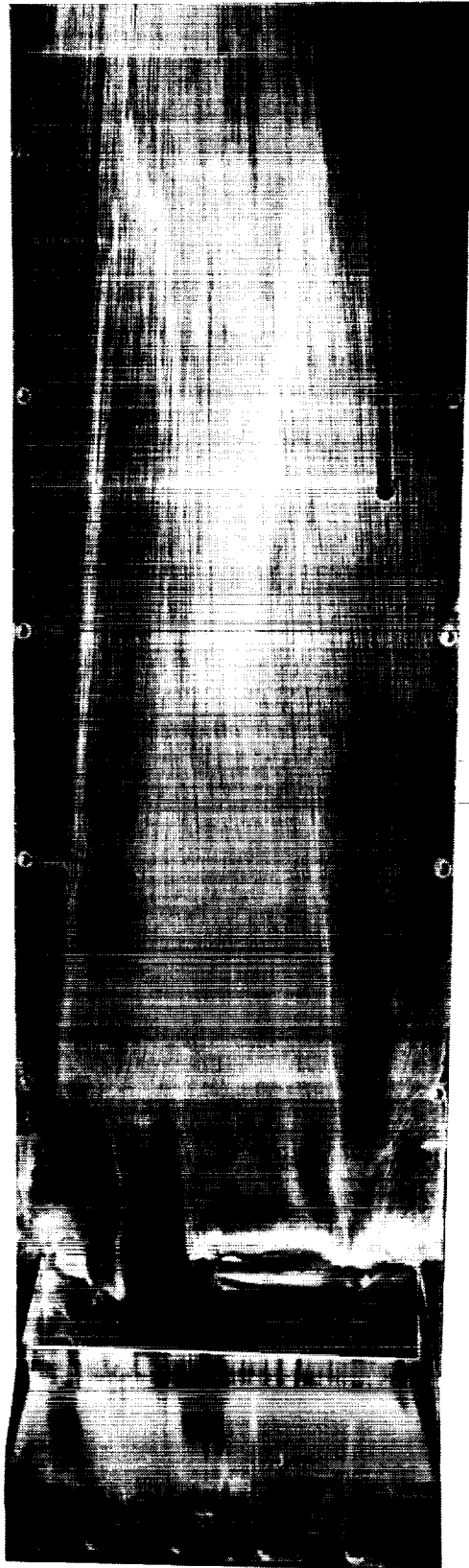
Figure 19. Oil flow photographs of model, off-design test conditions; P_{t_{co}} = 6895 \text{ kPa} , P_{t_j}/P_{t_{co}} = 154 , Run 17. (a) Ramp and cowl, top view.
