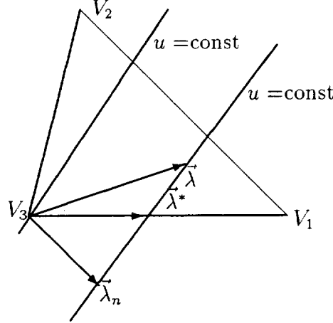
FIGURE 8. Construction of the NN scheme.
