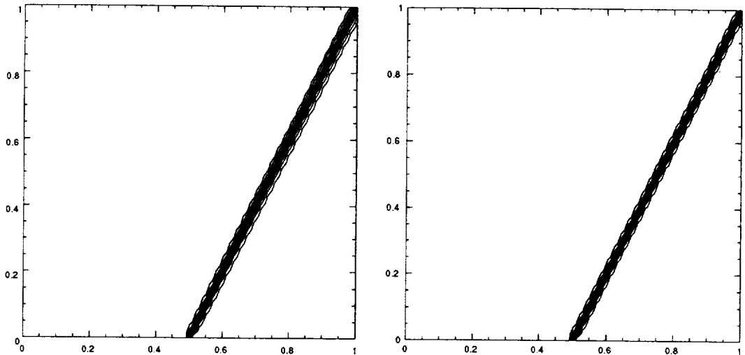
FIGURE 16. S and NNL scheme with Roe superbee limiter.
