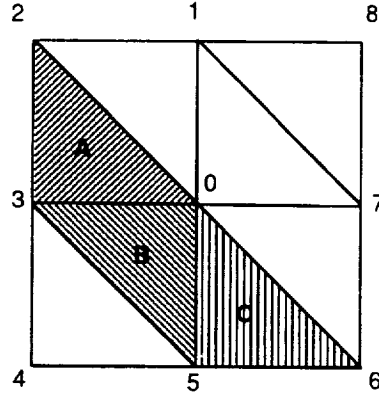
FIGURE 10. Possible triangulation of the Cartesian grid.
