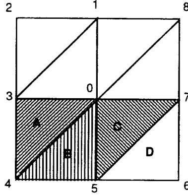
FIGURE 9. Possible triangulation of the Cartesian grid.
