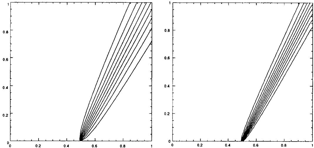
FIGURE 13. Regular upwinding and N scheme.
