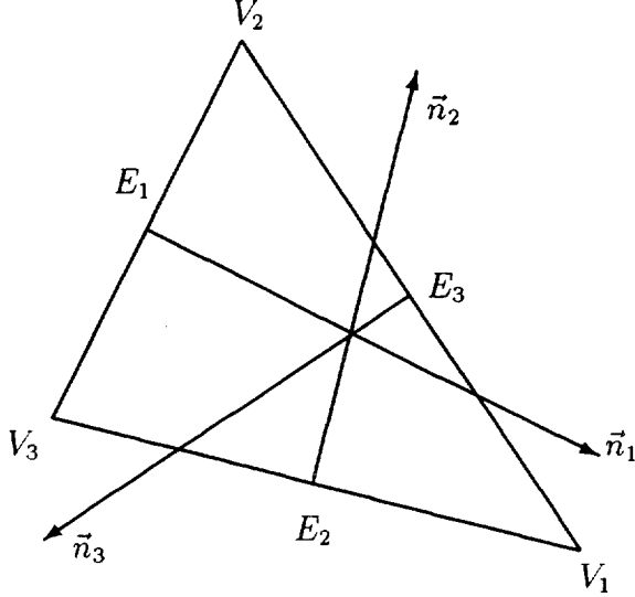
FIGURE 5. Illustration for construction of fluctuation-splitting schemes.
