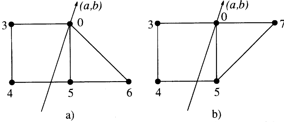
FIGURE 4. Positive (non-linear) zero cross-diffusion schemes: a) S scheme; b) S* scheme.
