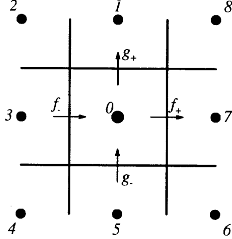
FIGURE 1. Control volume.
