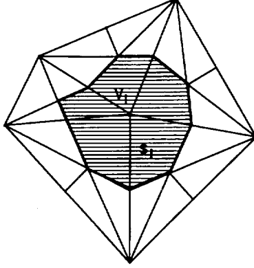
FIGURE 6. Median dual cell.
