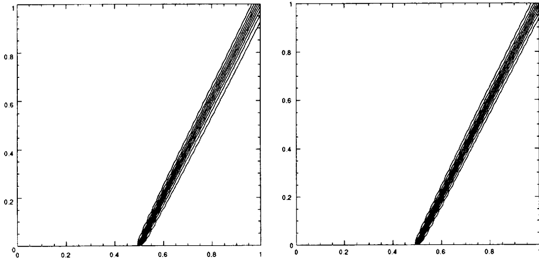
FIGURE 15. S and NNL scheme with van Leer limiter.
