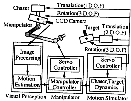
Fig. 9 System configuration of simulator
