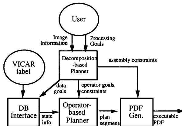
Figure 1: MVP Architecture
