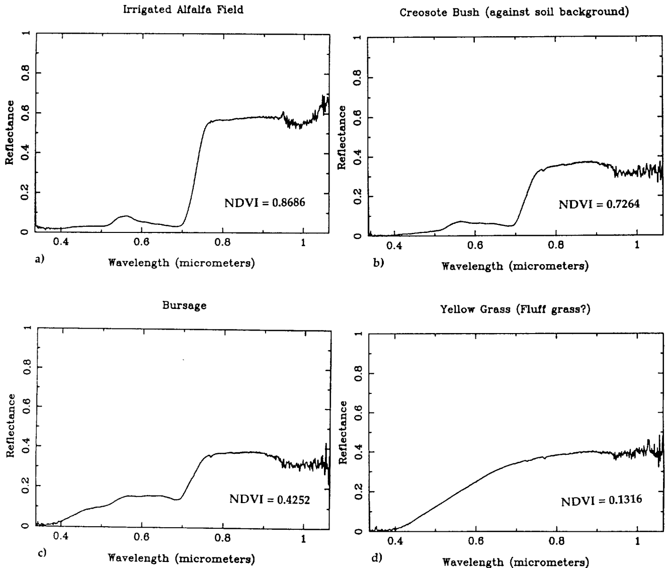
Figure 1: Spectra for some common Mojave Desert plant types and for an active irrigated alfalfa field in the Manix Basin area. In each case, the instrument field of view is completely filled by the vegetation being measured (100% vegetation cover). Compare the shapes of the spectra in the visible region and the nature of the red edge. NDVI values for each spectrum are listed to illustrate the poor performance of NDVI when looking at arid region vegetation. a) Irrigated alfalfa field. b) Creosote Bush. c) Bursage. d) An extremely common grass which is yellow most of the year; tentatively identified as fluff grass.
