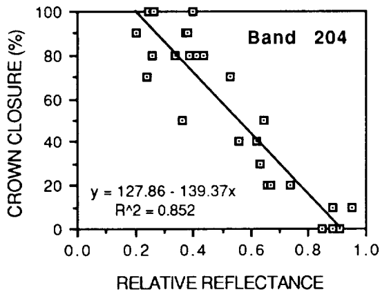
Figure 3: Crown closure as a function of the relative reflectance (atmospherically corrected data) for band 204 (2258.3 nm).
