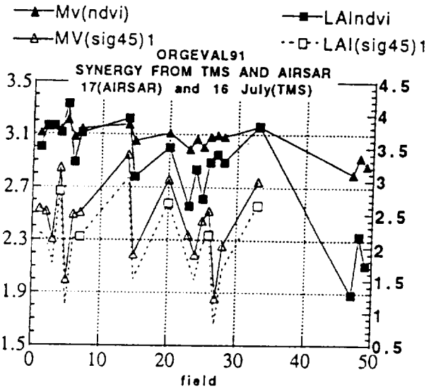
Figure 7: Simultaneous estimation of Leaf Area Index and vegetation water content from optical (TMS) and microwave (AIRSAR) images.
