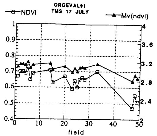
Figure 5: Spatial variations of NDVI and deduced vegetation water content M_v ( \text{kg/m}^2 ) over wheat fields.
