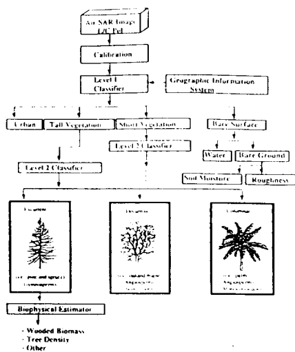
Figure 1. SAR terrain classifier
