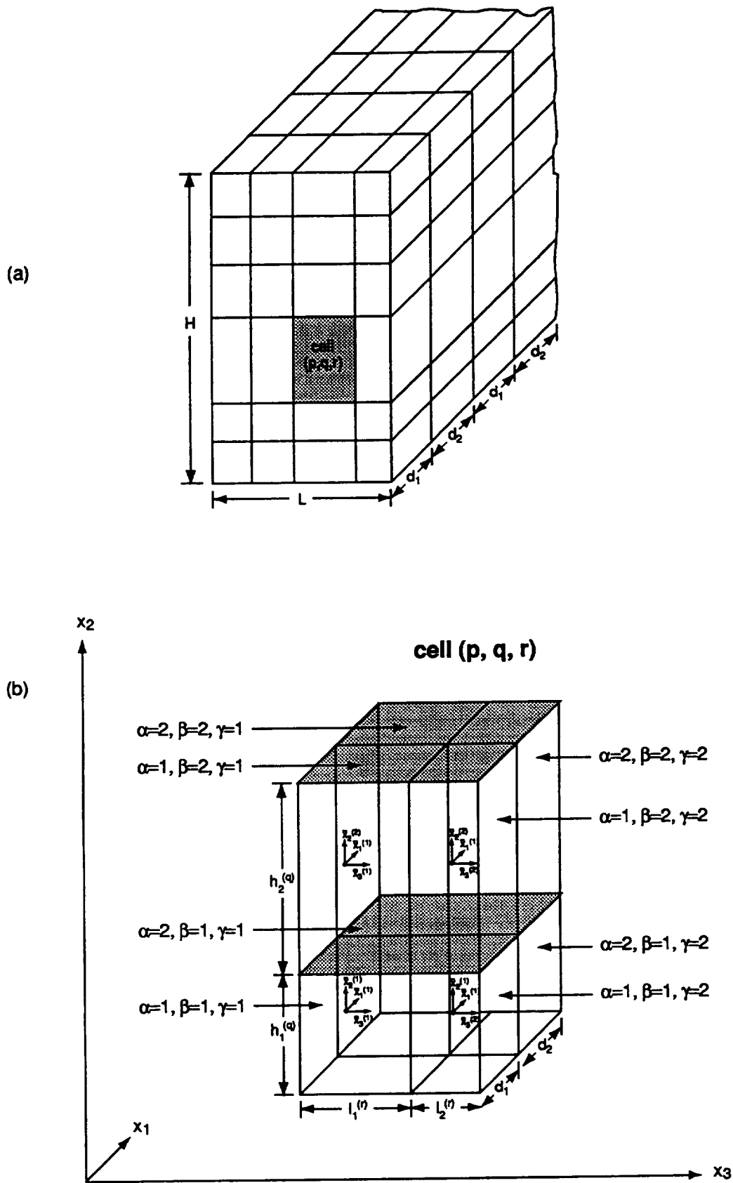
Figure 2 - (a) Three-dimensional schematic of a composite functionally graded in the x_2 and x_3 directions showing the dimensions of the basic building block (b) of the composite.
