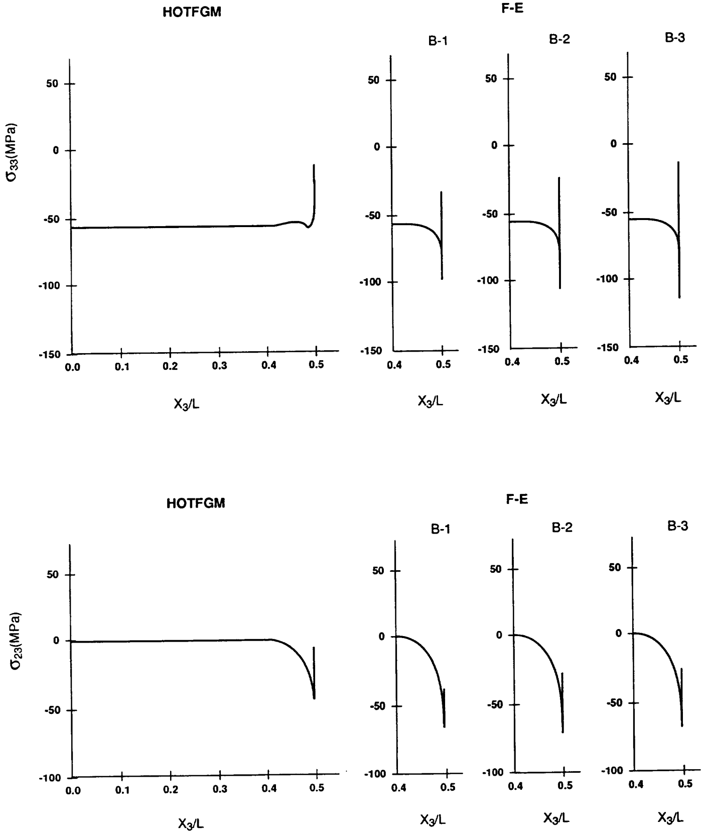
Figure 5 (cont'd) - Normal and shear stress distributions in the titanium ply at the interface separating B/Ep and Ti plies due to a temperature change of \Delta T = -154.45^\circ\text{C} . Comparison between the predictions of HOTFGM-2D and FE analysis.
