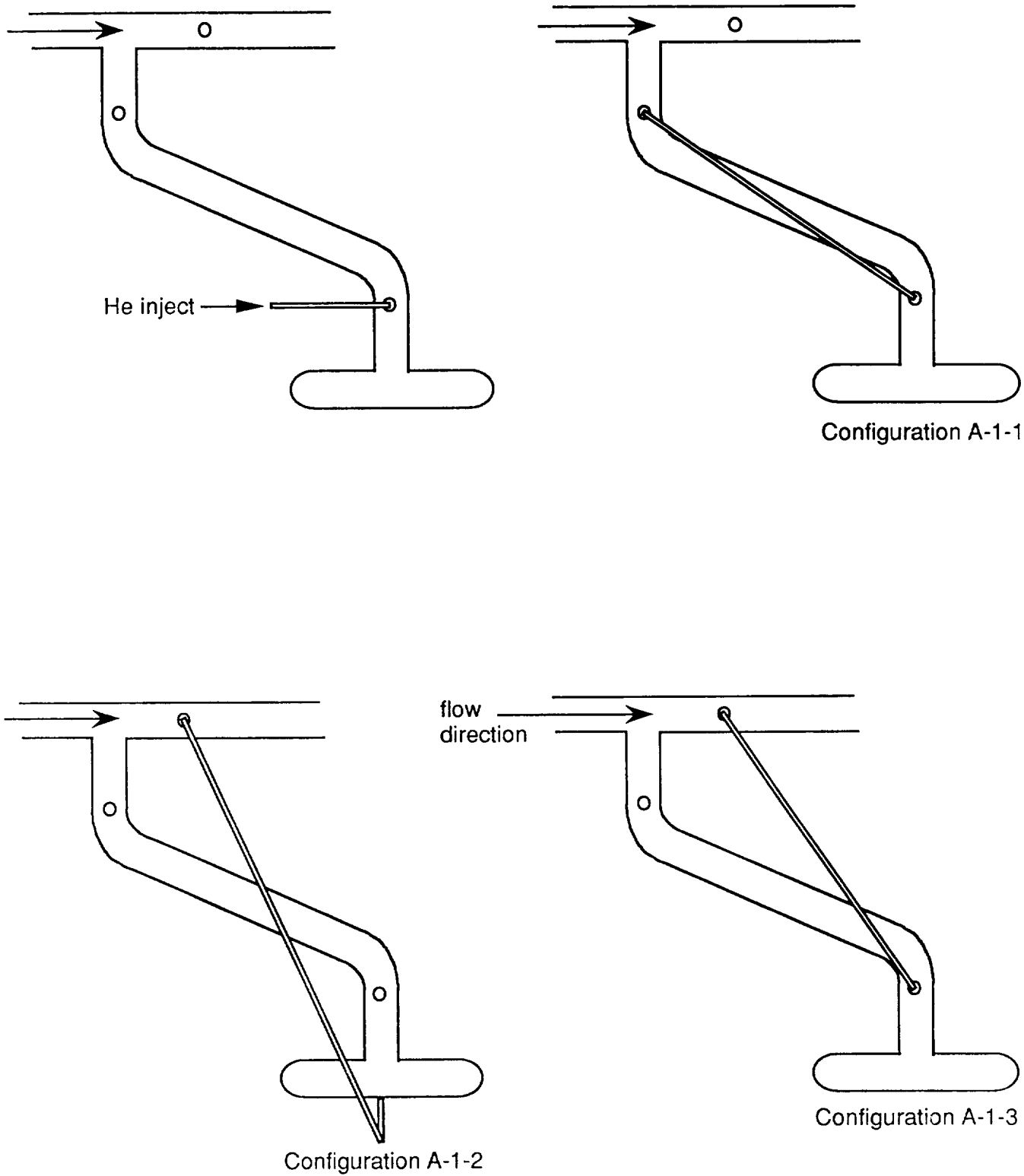
Figure 15. Helium bubbling and recirculation line configurations.
