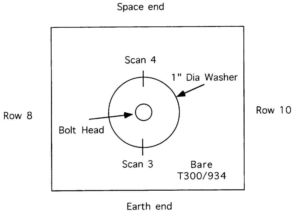
Figure A-1. Location of profilometer scans 3 and 4 taken through the washer protected area and adjacent exposed areas in the bare T300/934 quadrant of the panel on tray D9.
