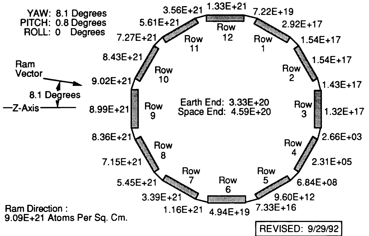
Figure 2. Atomic Oxygen Fluences for all Row, Longeron, and End-bay Locations of LDEF.
