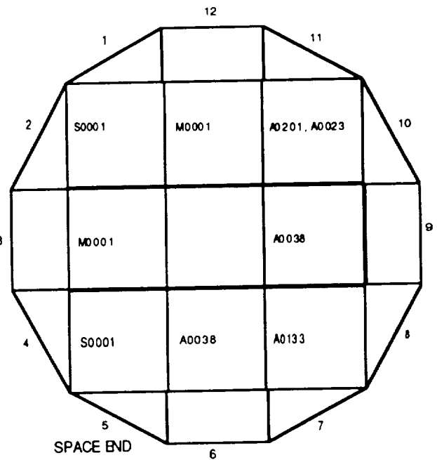
Figure 1. Schematic Diagram of the Location(s) of each LDEF Experiment.
