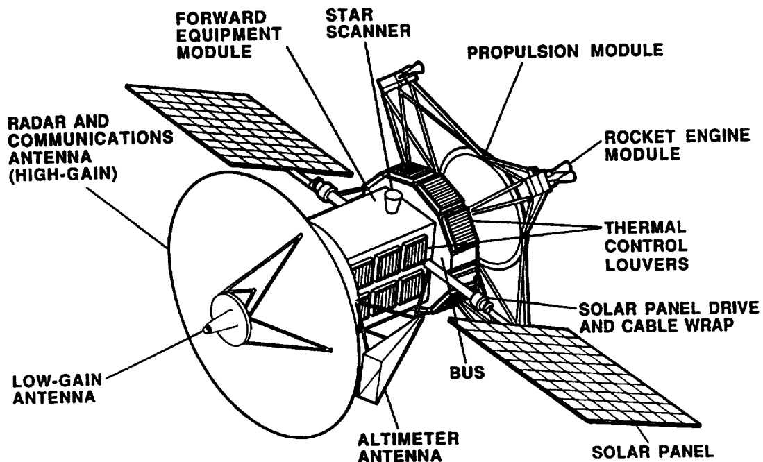
Figure 2.1. The Magellan Spacecraft.
