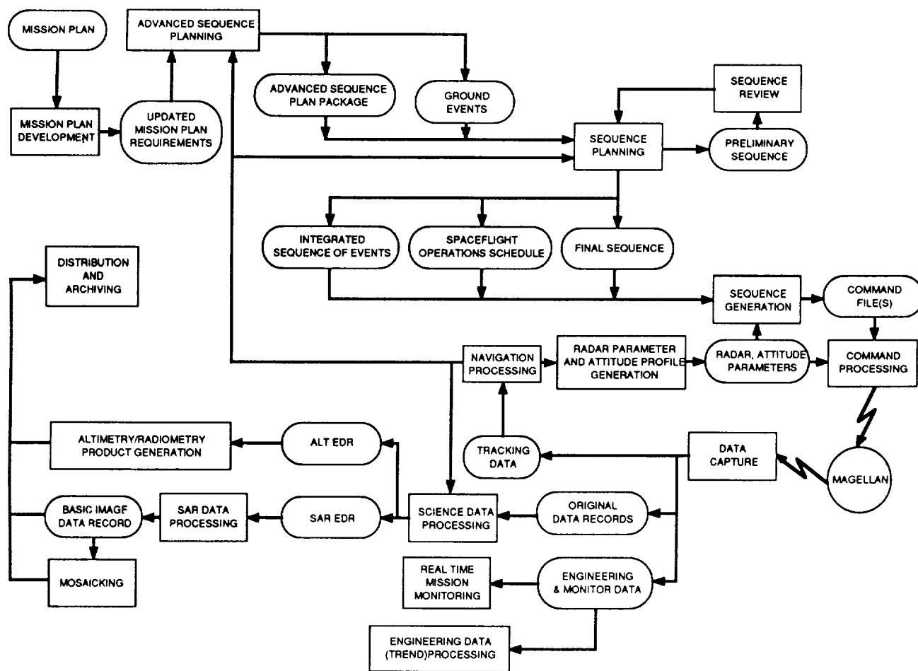
Figure 5.1. Uplink and Downlink Processes.
