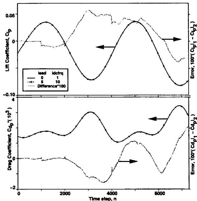
Fig. 13: Oscillating Airfoil case: Lift, C_{lp} , and drag, C_{dp} , history
