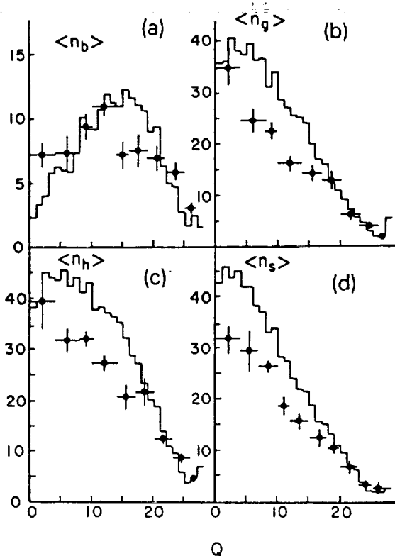
Fig. 5. Correlation functions versus Q in Fe + AgBr interactions: (a) \langle n_b \rangle ; (b) \langle n_g \rangle ; (c) \langle n_h \rangle and (d) \langle n_s \rangle . The dots are experimental data. The histograms are the DCM calculation results.
