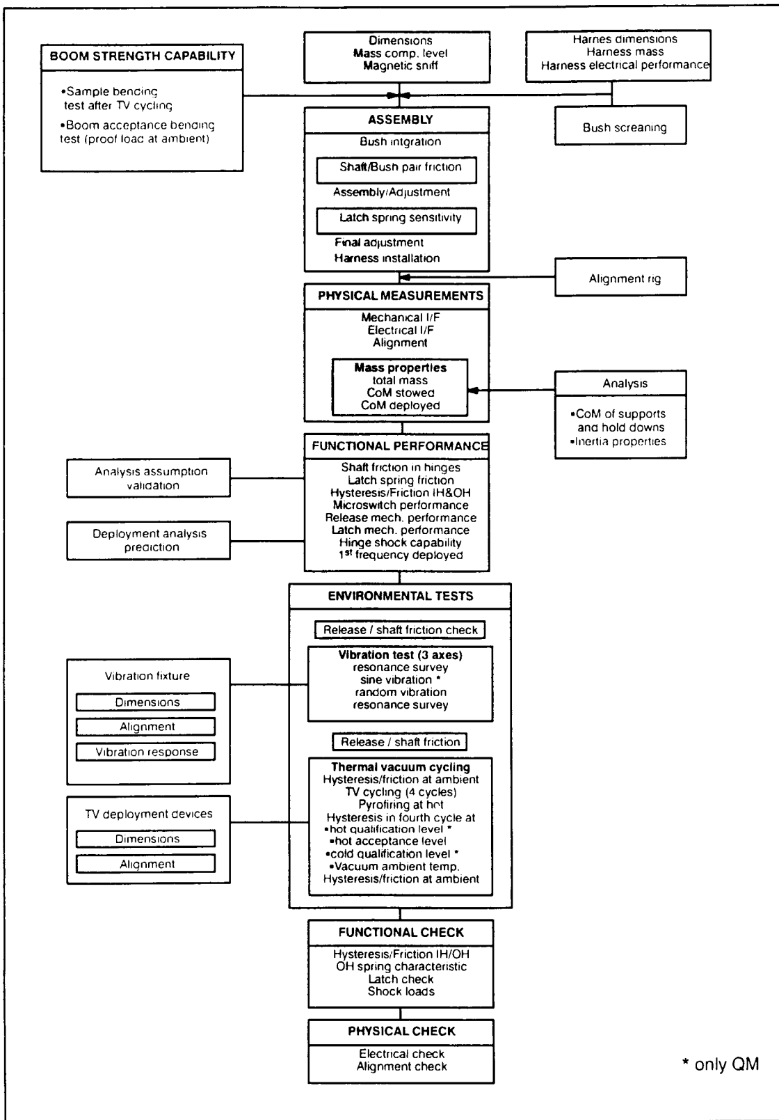
Figure 6 RB Test flow
