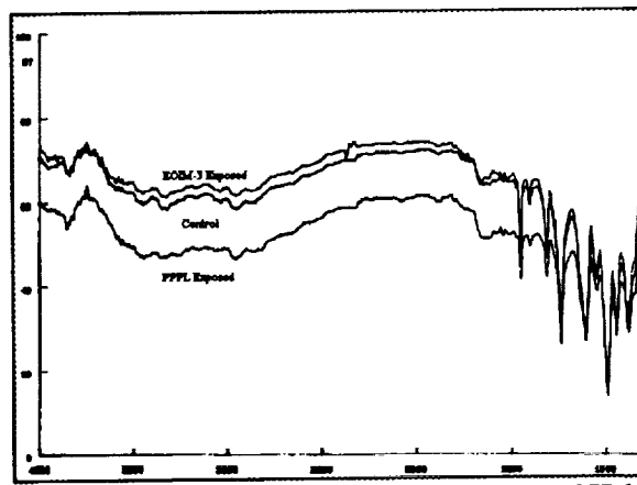
Figure 7. FTIR of EOIM-3 and PPPL exposed Halar showing percent transmission as a function of wavenumber ( \text{cm}^{-1} ).
