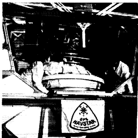
MLI Blankets and Heaters
