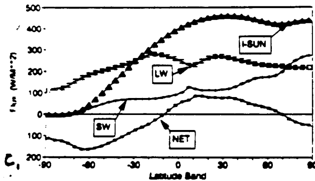
Figure 1. Nimbus-7 scanner (MLCE) emitted longwave (LW), reflected shortwave (SW), net radiation (NR), and top-of-the-atmosphere insolation, I(sun): (a) annual average (June 1979 through May 1980), and seasonal averages (b) December through February, (c) June through August.
