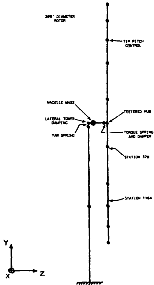
Figure 3. MOD2 finite element model.
