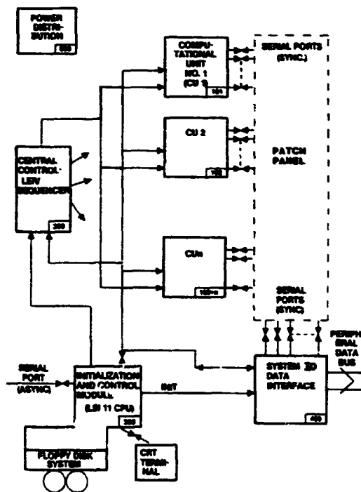
FIGURE 1 CAPPS SYSTEM LOGIC DIAGRAM
