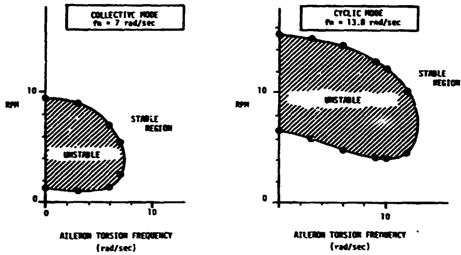
Figure 12. MCD-5A Flutter Boundaries Unbalanced Aileron .725P - 1.0P Shown as a Function of Aileron Torsional Frequency
