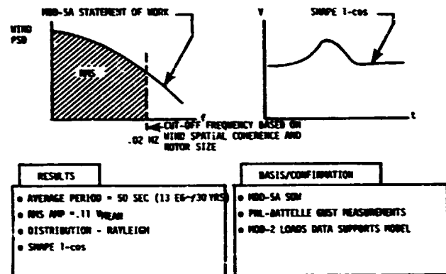
Figure 4. Development of Large Rotor-Enveloping Gust Model
