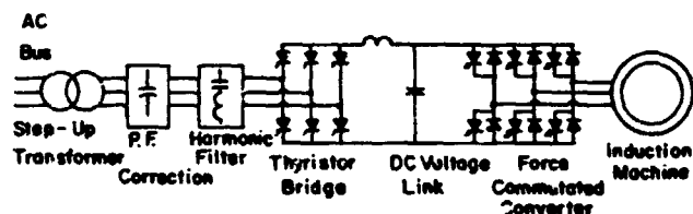
Fig. 11 Induction Generator with DC Voltage Link and AC/DC/AC Conversion
