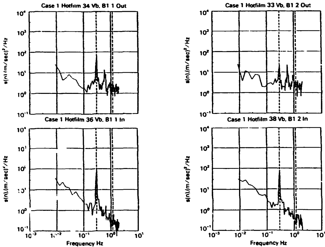
Figure 16--Power spectral density functions of rotationally measured axial wind speed at four diametral locations, for MOD-2 #2 wind turbine. Neutral case.
