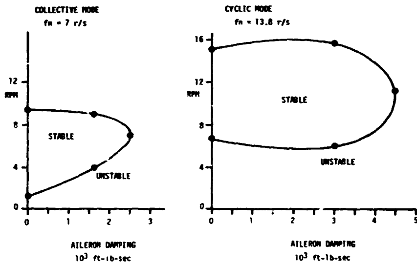
Figure 13. MCD-5A Flutter Boundaries Unbalanced Aileron .725P - 1.0P Shown as a Function of Aileron Damping
