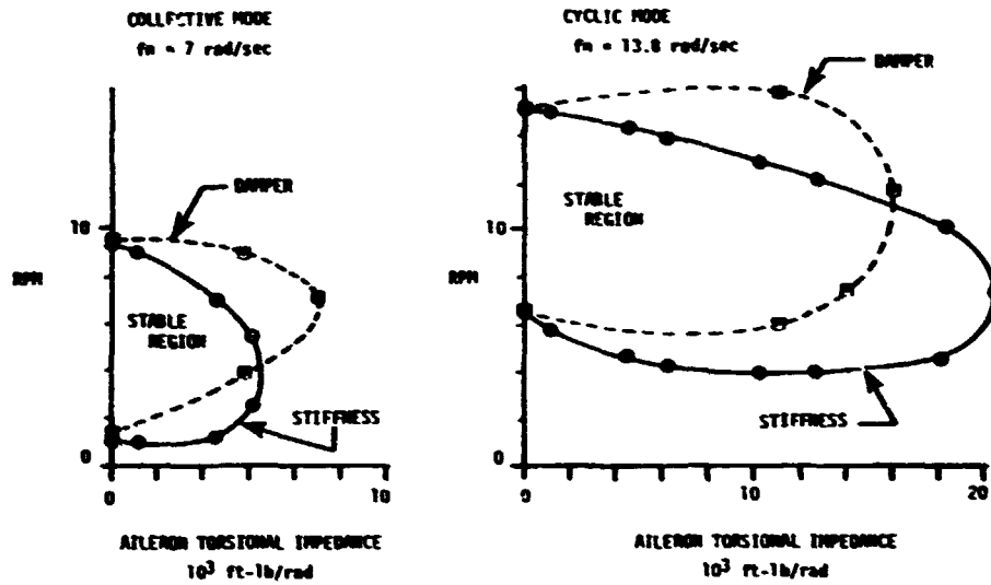
Figure 14. MDL-5A Flutter Boundaries Unbalanced Ailerons .725P - 1.0P Shown as a Function of Aileron Torsional Impedance
