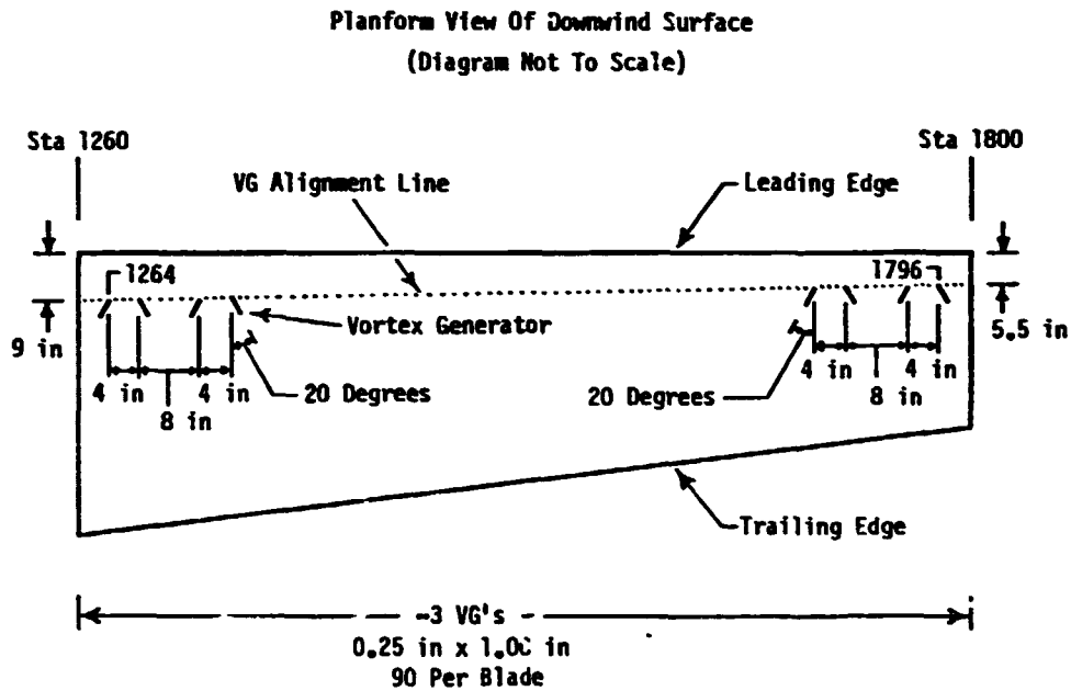
Figure 8. Vortex Generator Installation On Mod-2 Blade Tip Assembly.
