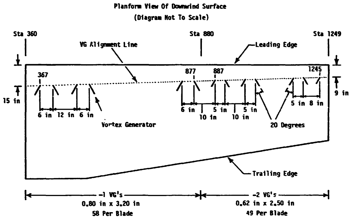
Figure 7. Vortex Generator Installation On Mod-2 Mid-blade Assembly.
