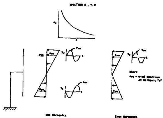
Figure 30. Conceptual Description of the NASA Interim Turbulence Model
