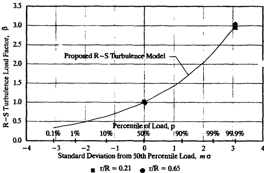
Figure 15. Proposed model of the R-S turbulence load factor with which the spectrum of cyclic flatwise bending loads on a HAWT blade can be calculated from the 50th percentile level of load. The model is based on a log-normal probability distribution.
