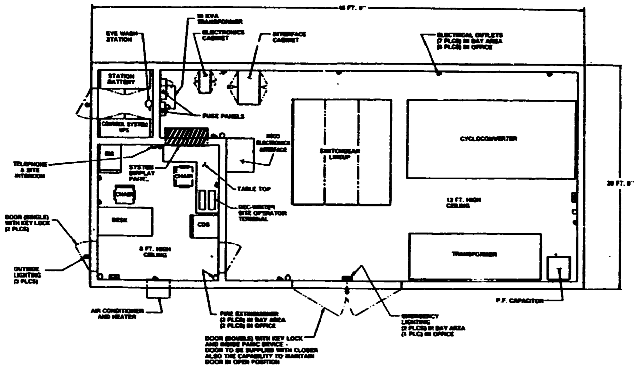
Figure 14- Electrical Equipment Building
