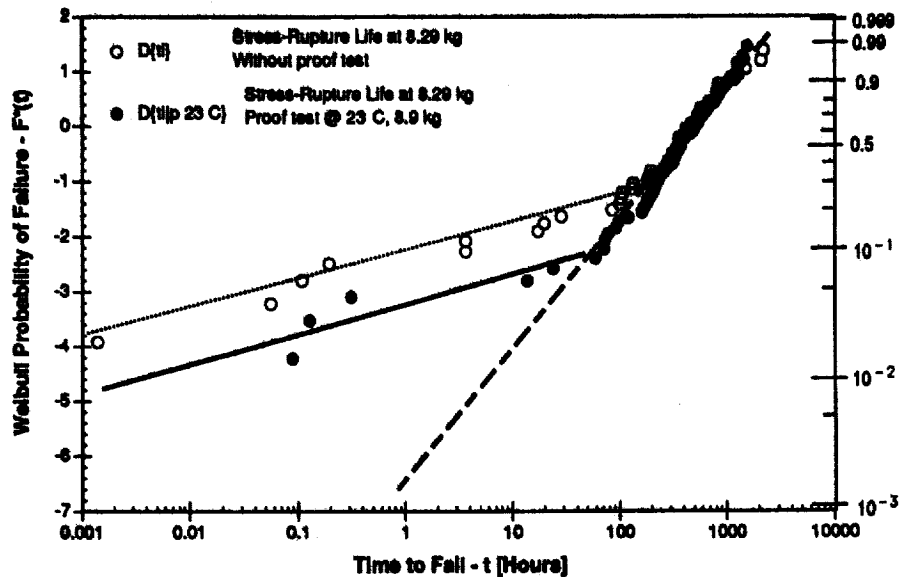
Figure 5. Life of aramid-epoxy composite under sustained load( 8.29 kg) after survival of preload (8.93 kg) at 23°C.
