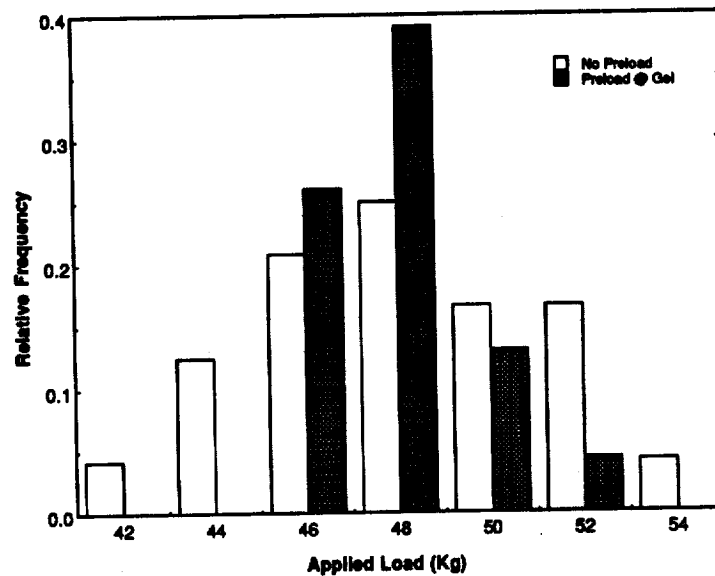
Figure 9. Distribution free strength comparisons of graphite-epoxy composite versus composite preloaded at gel state during fabrication.
