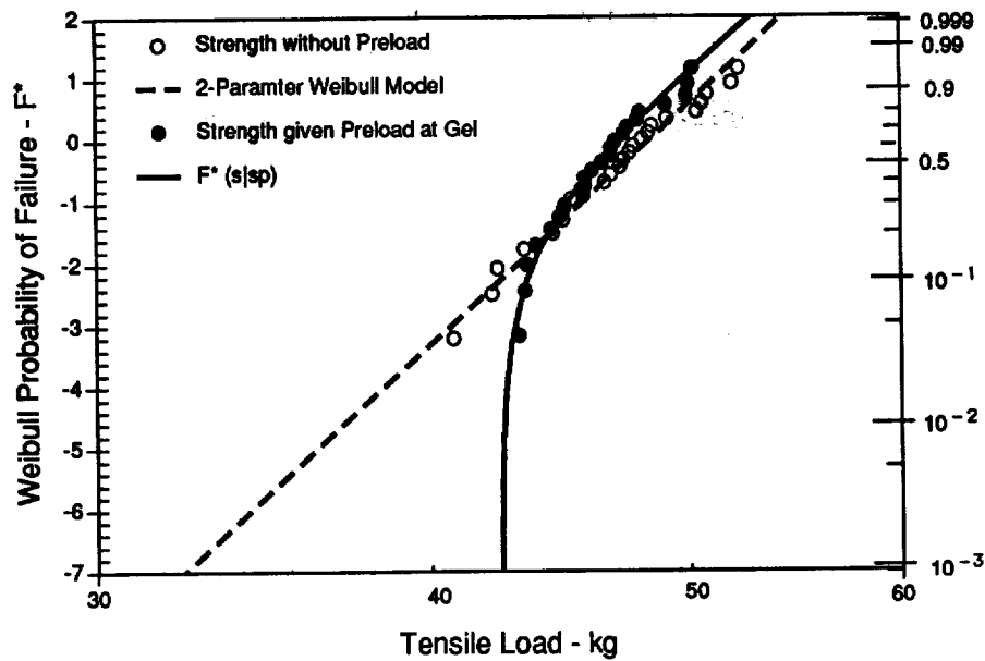
Figure 8. Strength of graphite-epoxy composite versus strength of composite preloaded at gel state during fabrication.
