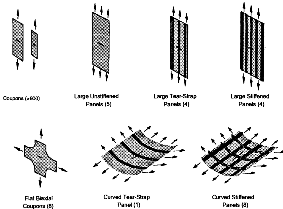
Figure 1. ATCAS tension fracture testing.
