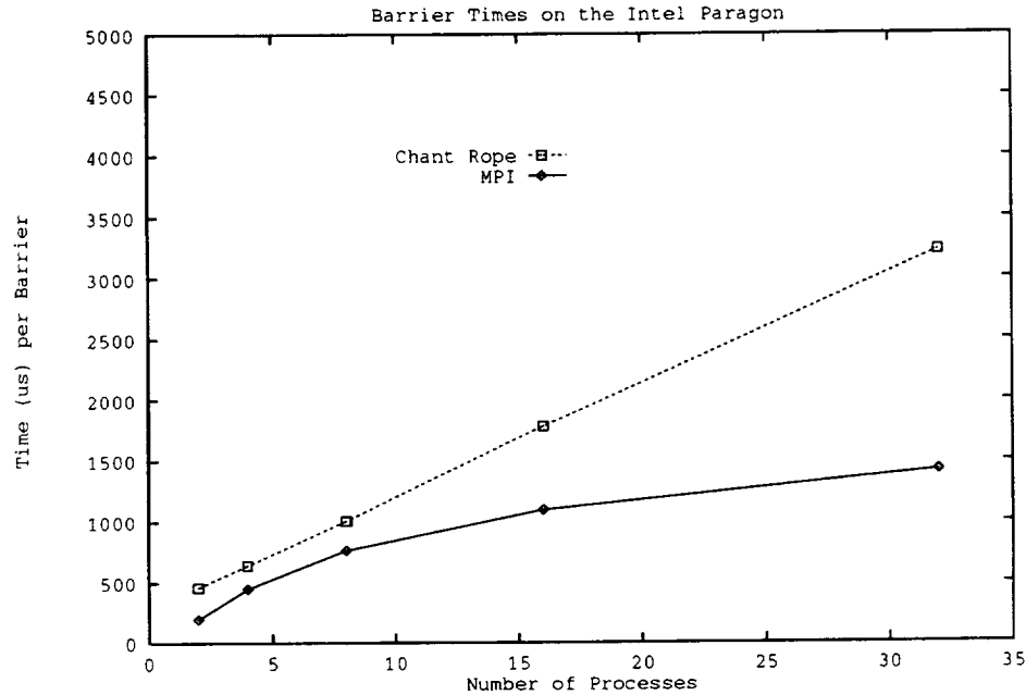
Figure 8: Execution times for barrier
