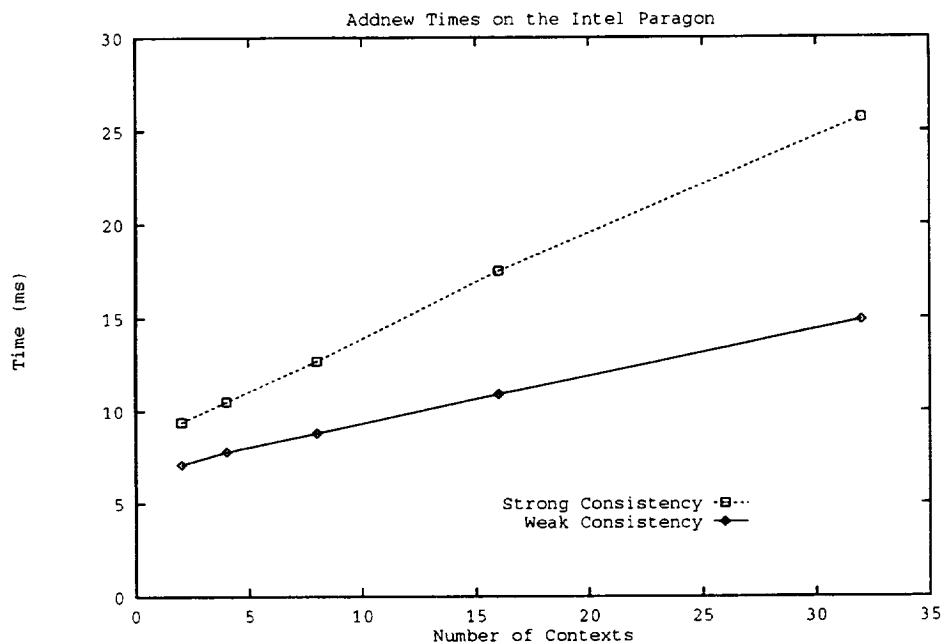
Figure 6: Execution times for rope_addnew , 4 threads per context
