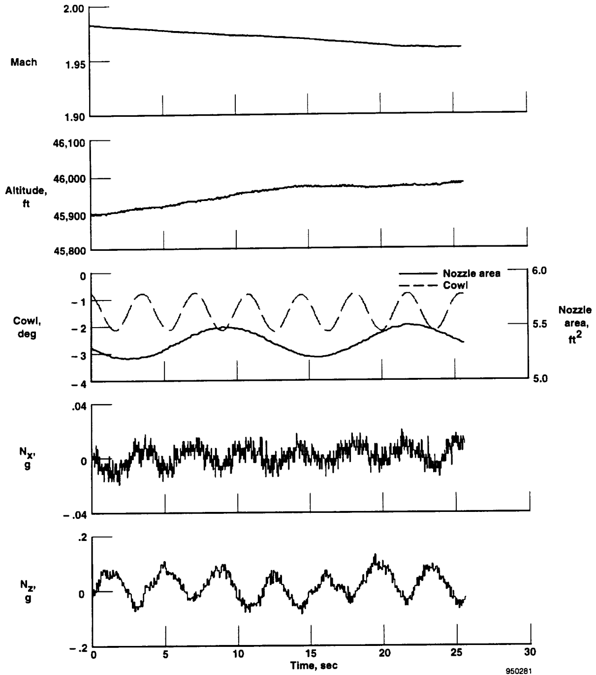
Fig. 5. Time histories of simultaneous nozzle area and cowl excitation.
