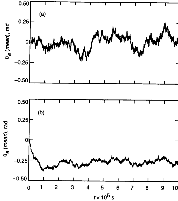
Fig. 10. \theta_e (mean) of balanced and unbalanced data streams: (a) balanced data stream ( \rho = 0.5 ): mean of phase error is centered at zero and (b) unbalanced data stream ( \rho = 0.6 ): mean of the phase error deviates away from zero.
