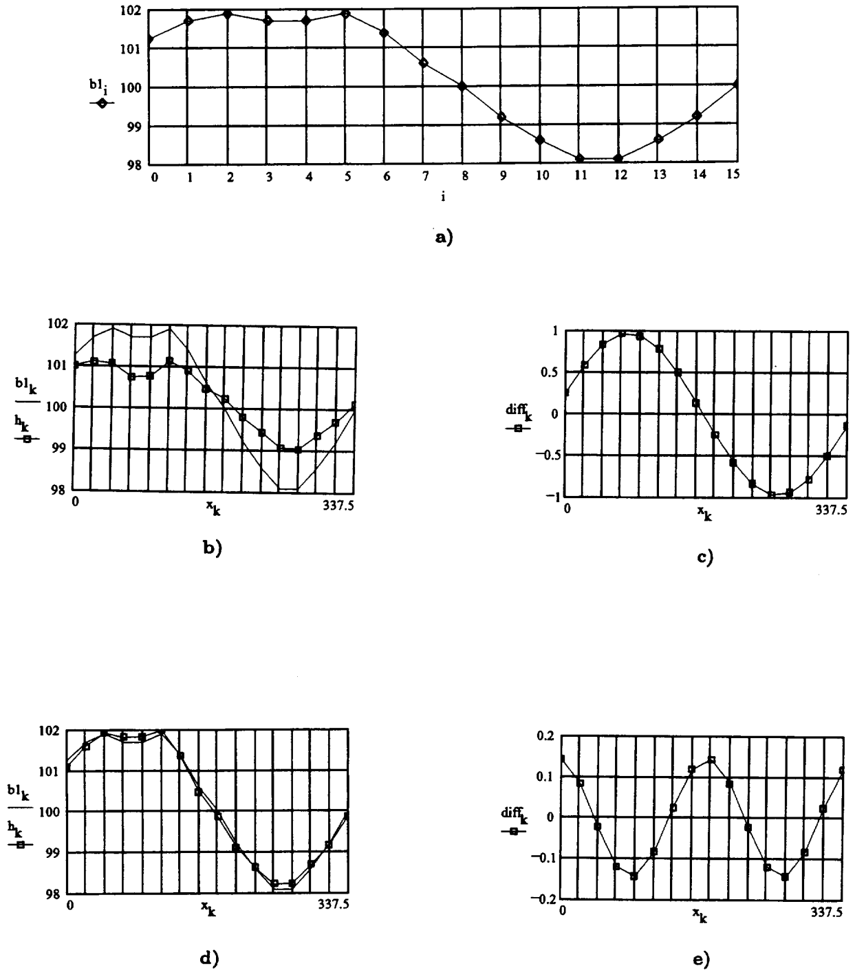
Fig. 6. Polarization measurements for SeaWiFS band 1. a) The instrument response measured at 22.5° increments of polarizer rotation. These values are the input values for Fourier analysis. b) The polarization values with and without the one-cycle component b1(k) equal the measured values, and h(k) equal the measured values without the one-cycle component. c) The one-cycle polarization component generated by Fourier analysis. d) The polarization values with and without the two-cycle component b1(k) equal the measured values and h(k) equal the measured values without the two-cycle component. e) The two-cycle polarization component generated by Fourier analysis.
