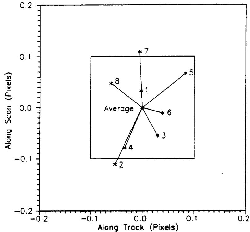
Fig. 5. Band-to-band registration of SeaWiFS. The locations of the individual band centers are given relative to the average for the eight bands. The distances are given in “pixels,” where 1 pixel equals 1.6 mrad. The figure also includes a square that is 0.1 pixel on each side and which is centered on the average center location for the eight bands.
