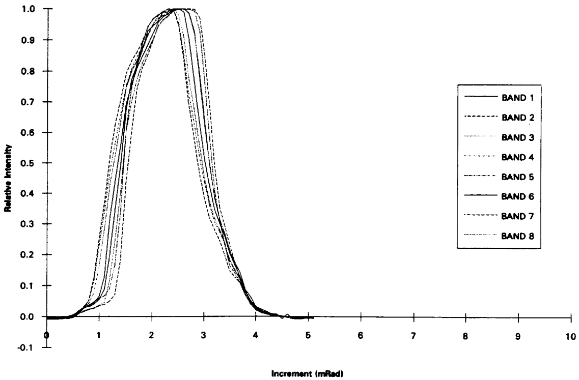
Fig. 1. The along-scan and along-track line spread functions. The top figure shows the along-scan line spread function. In this figure, the zero offsets have been removed from the data, and the results have been scaled to unity. The bottom figure shows the along-track line spread function. As in the top figure, the zero offsets have been removed from the data, and the results have been scaled to unity.
