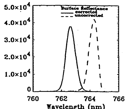
Figure 6. Oxygen band center histograms for the full Blackhawk Island scene, corrected and uncorrected for surface reflectance.
