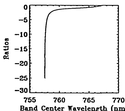
Figure 5. Ratios of two sides of the oxygen feature for 100 different sensor wavelength calibrations.
