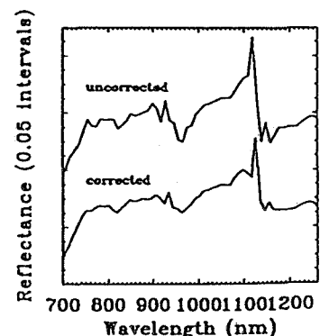
Figure 9. Reflectance spectra in AVIRIS spectrometer B calculated using ATREM from Gainesville, Florida. Wavelengths for the corrected spectrum were shifted by 2.8 nm.
