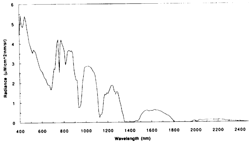
Figure 2. Upwelling spectral radiance measured by AVIRIS for the Old Jack Pine site on 21 July 1994.
