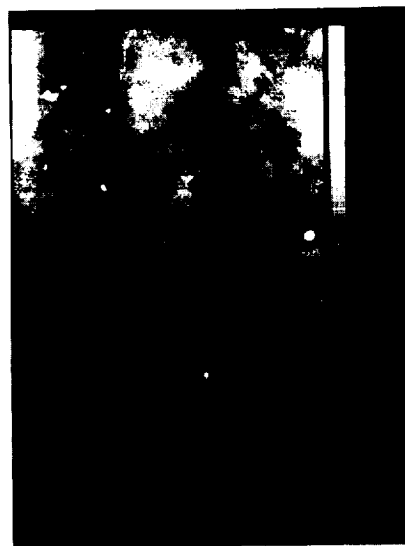
Figure 4. Image of water vapor over the SSA Old Jack Pine site (see AVIRIS Workshop Slide 3).
