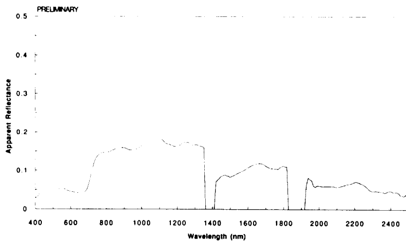
Figure 7. RTC-derived surface reflectance for SSA Old Jack Pine site, from AVIRIS on 21 July 1994.
