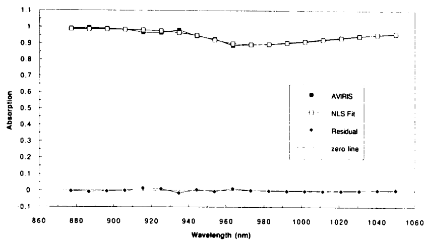
Figure 5. Nonlinear least squares spectral fit for determination of absorption due to leaf liquid water.
