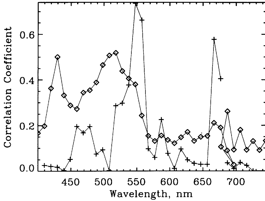
Figure 2. Spectral variation of the r^2 for the AVIRIS reflectance at single bands ( \diamond ) and first difference of the AVIRIS reflectance with gap 1 (+).
