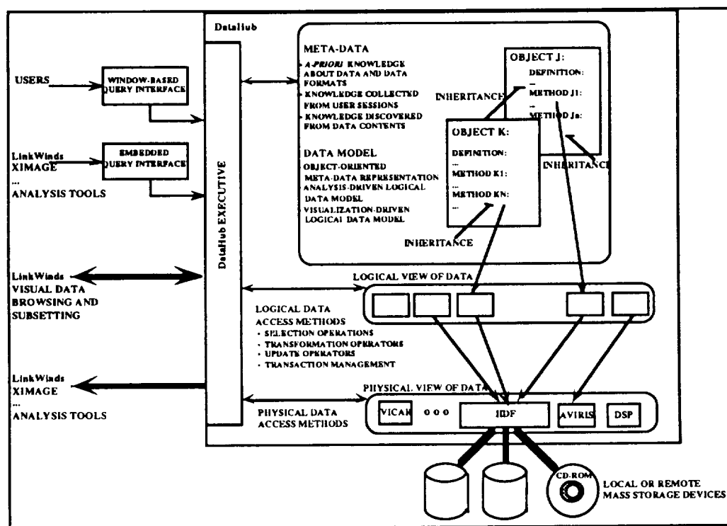
Figure 1 -- Functional Architecture
