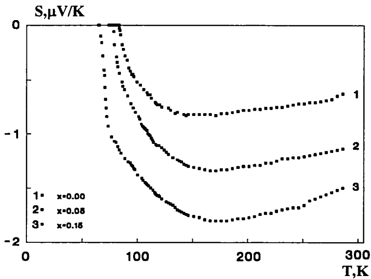
Fig.2. The thermopower vs. temperature for \text{Y}_{1-x}\text{Ca}_x\text{Ba}_2\text{Cu}_3\text{O}_y
