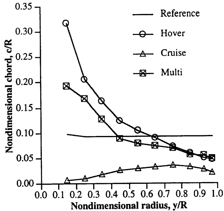
Figure 7 Chord distributions
