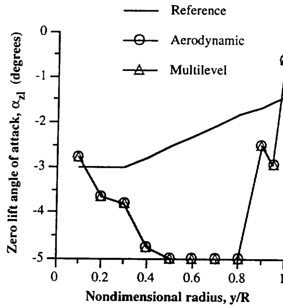
Figure 31 Zero lift angle of attack distributions
