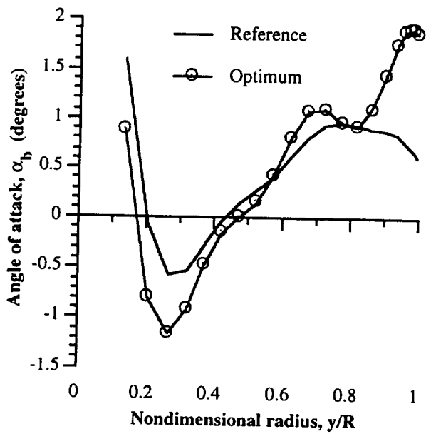
Figure 48 High speed cruise angle of attack distribution
