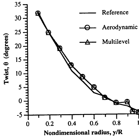
Figure 30 Blade twist distributions
