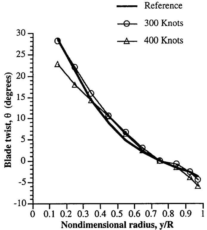
Figure 17 Twist distributions
