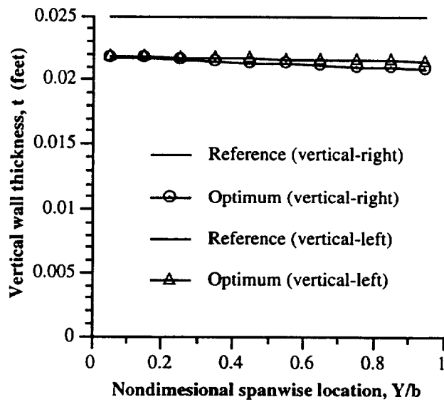
Figure 51b Vertical wall thicknesses distributions
