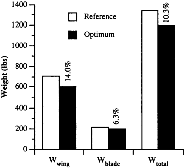
Figure 45 Optimum structural results
