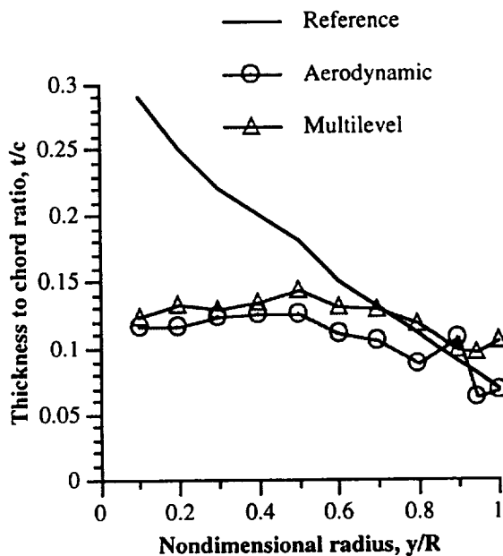
Figure 27 Thickness to chord ratio distributions
