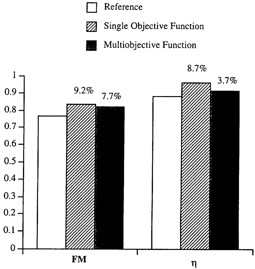
Figure 6 Summary of optimum results
