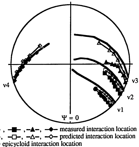
Fig. 7 Blade vortex interaction locations in the plane of the rotor for the AH-1/OLS model rotor.
