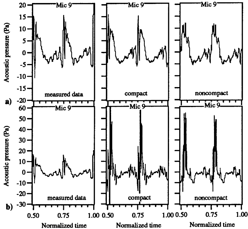
Fig. 11 Acoustic pressure is plotted as a function of normalized time (1 rev = 1 unit of time), row a) measured acoustic data compared to acoustic prediction using compact and non-compact formulations with measured surface pressure, row b) measured acoustic data compared to acoustic prediction using compact and non-compact formulations with FPR predicted surface pressure.
