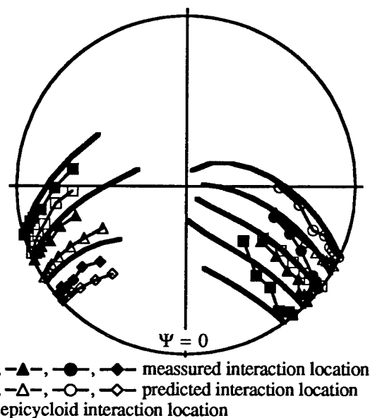
Fig. 9 Blade vortex interaction locations in the plane of the rotor for the UH60 model rotor.
