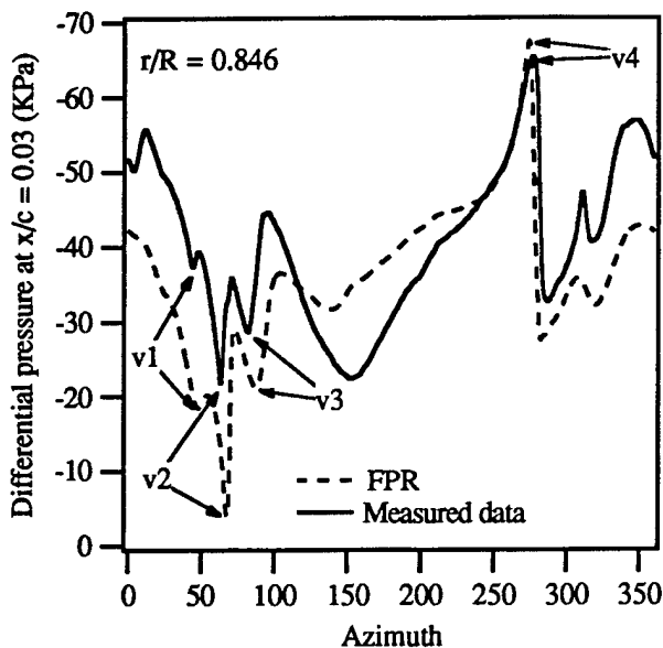
Fig. 6 Leading edge differential pressure as a function of azimuth for the AH-1/OLS model rotor. The vortex locations of interest are labeled for the measured data and the FPR prediction with a/c = 0.20
