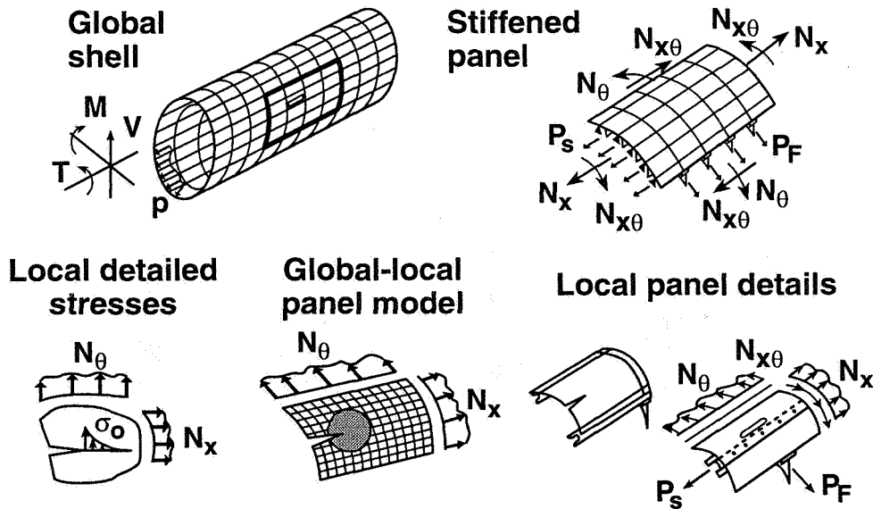
Figure 8. Hierarchical nonlinear stiffened shell models.
