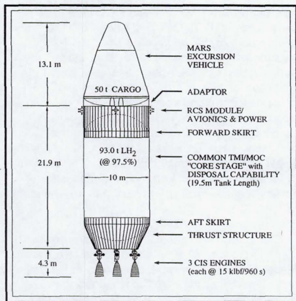
Fig. 18. Mars Cargo Vehicle and Mass Properties
