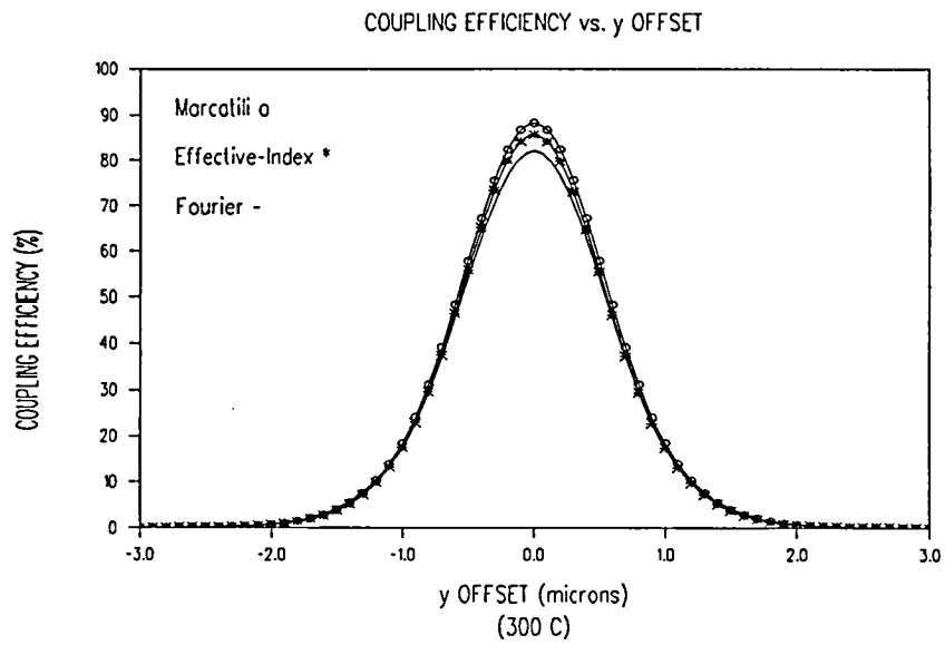
Figure 5.51: Calculated coupling efficiency vs. y offset at 300^{\circ}\text{C} .
