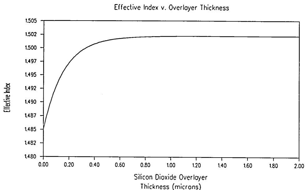
Figure 3.6: Guide effective index calculated for various SiO 2 overlayer thicknesses.
