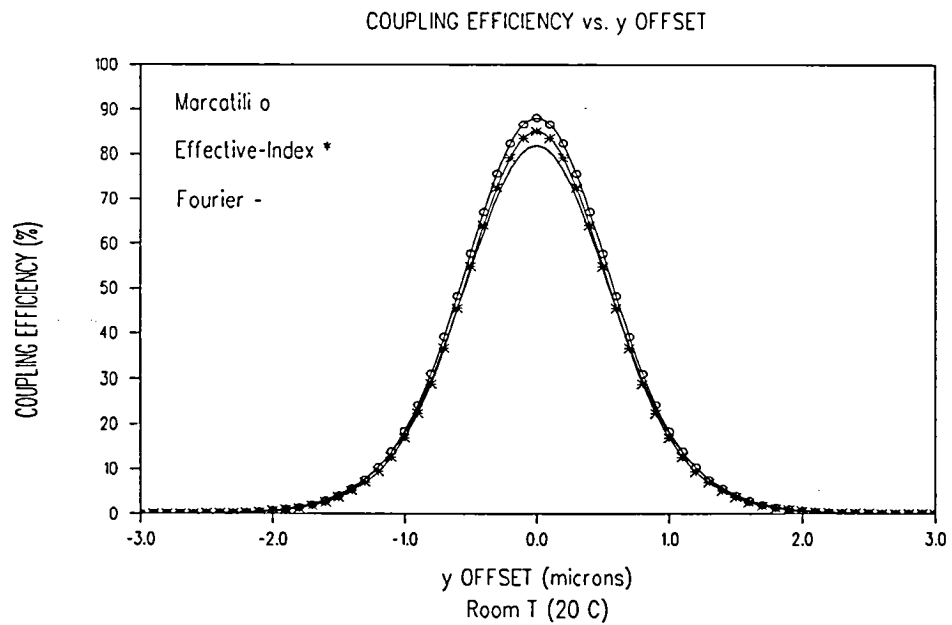
Figure 5.43: Calculated coupling efficiency vs. y offset.
