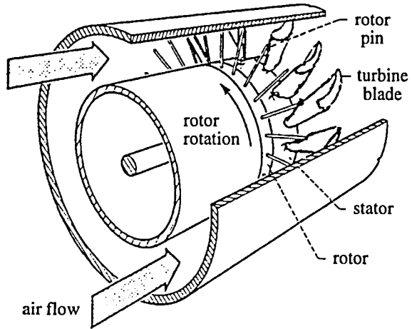
Figure 1 - Rotor-Wake Facility schematic
