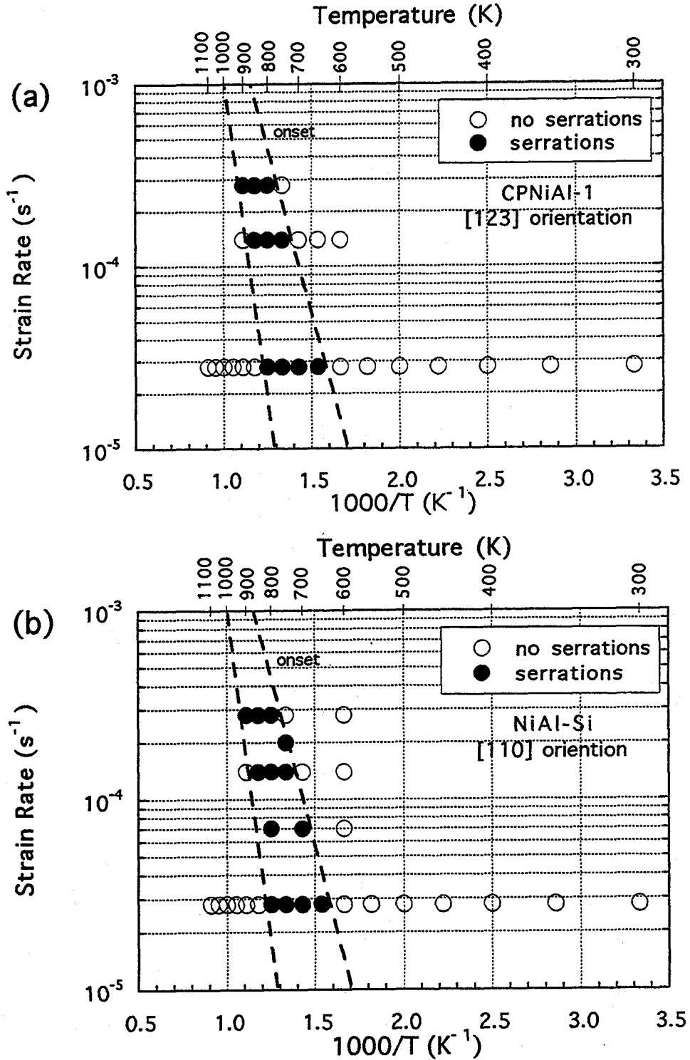
Figure 58. Plots of \ln \dot{\epsilon} versus 1/T for CPNiAl-1 and NiAl-Si illustrating the T - \dot{\epsilon} regimes for serrated flow. (a) CPNiAl-1 and (b) NiAl-Si.
