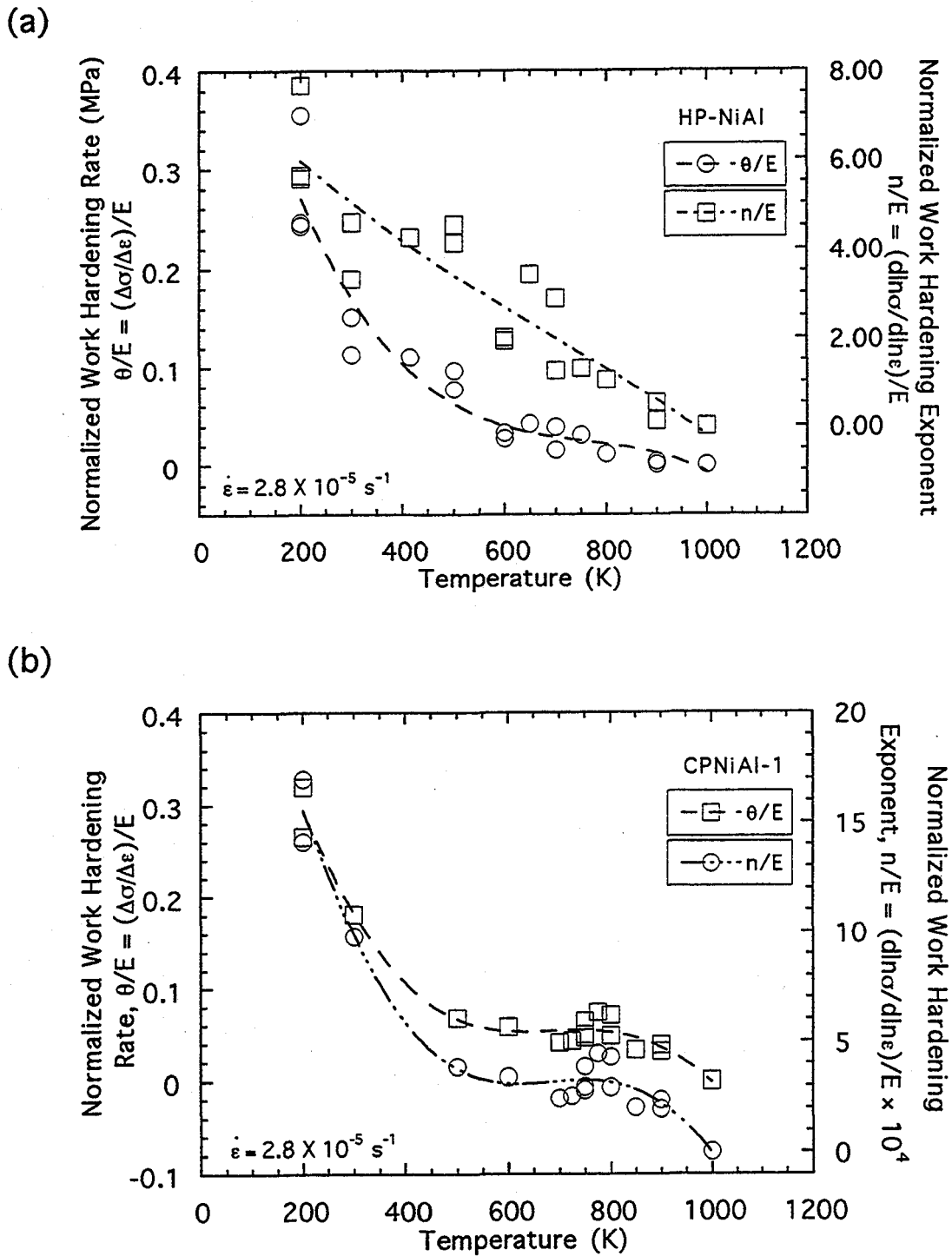
Figure 54. Temperature dependence of the normalized work hardening rates, \theta/E , and work hardening exponents, n/E , for NiAl single crystals: (a) HP-NiAl; (b) CPNiAl-1; (c) CPNiAl-2; (d) NiAl-Mo; (e) UF-NiAl1; and (f) NiAl-Si.
