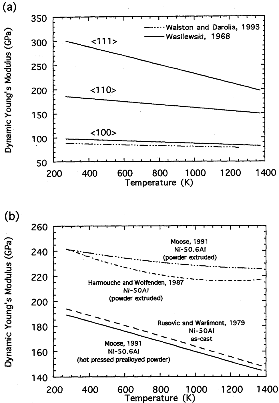
Figure 4. Elastic properties of single crystal and polycrystalline NiAl alloys: (a) single crystal NiAl as a function of orientation and temperature; (b) polycrystalline NiAl as a function of processing route and temperature (Data compilation from [7]).
