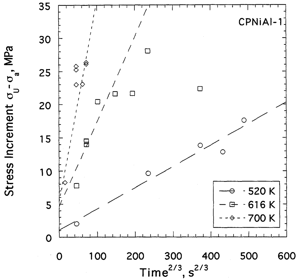
Figure 42. Plots of \Delta\sigma_u vs. t^{2/3} for CPNiAl-1 aged at 520, 616, and 700 K.
