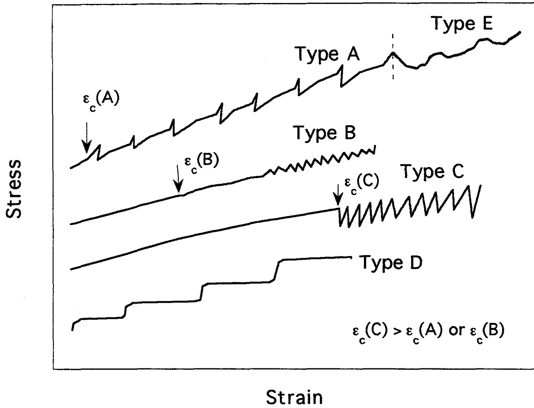
Figure 12. Examples of the different types of flow stress serrations observed during dynamic strain aging (after [106]).
