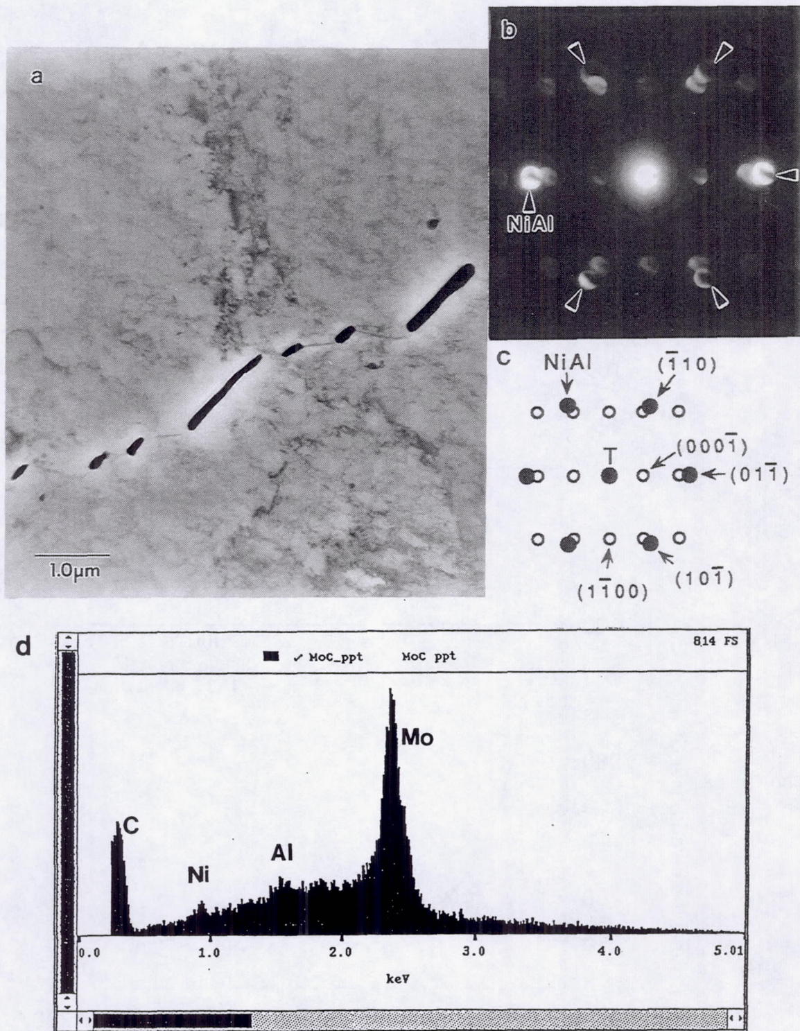
Figure 52. Precipitates observed in NiAl-Mo: (a) BFTEM micrograph of Mo 2 C precipitates in NiAl-Mo; (b) TEM microdiffraction pattern illustrating an orientation relationship ( [111]_{\text{NiAl}} // [11\bar{2}0]_{\text{Mo}_2\text{C}} and (01\bar{1})_{\text{NiAl}} // (000\bar{1})_{\text{Mo}_2\text{C}} ) between the Mo 2 C precipitate and NiAl matrix; (c) a schematic representation of (b); and (d) SEM EDS spectra for one of the precipitates indicating that they are indeed Mo 2 C.
