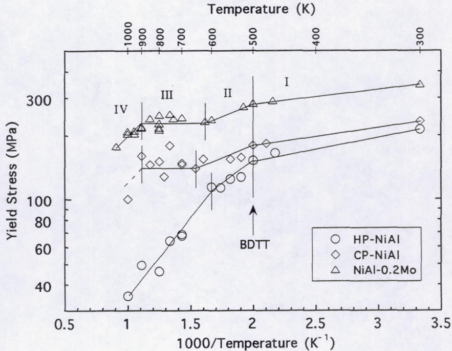
Figure 14. The temperature dependence of the 0.2% offset yield stress for HP-NiAl, CP-NiAl, and NiAl-0.2Mo single crystals and additional data from the literature.
