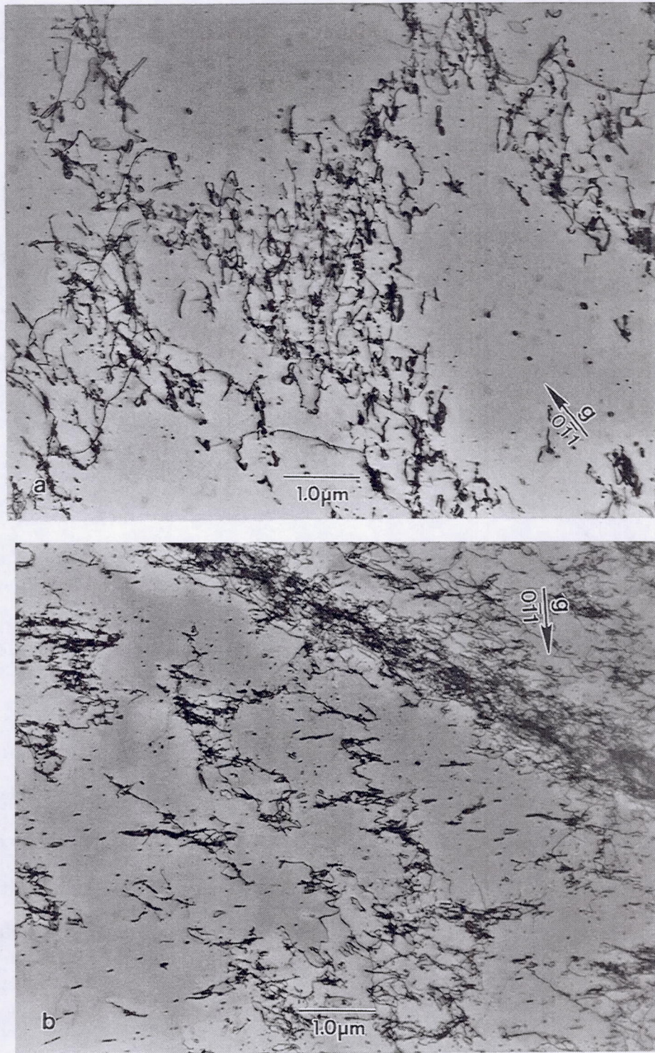
Figure 64. Deformation structure observed in HP-NiAl after 9% plastic deformation at 725 K. (a) Cellular morphology observed in most samples and (b) a single deformation band observed in one of the foils.
