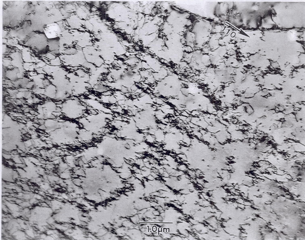
Figure 51. BFTEM of dislocation structure observed in NiAl-100C after 11.5% deformation at 800 K illustrating the transition of a dislocation cell structure to a banded structure.
