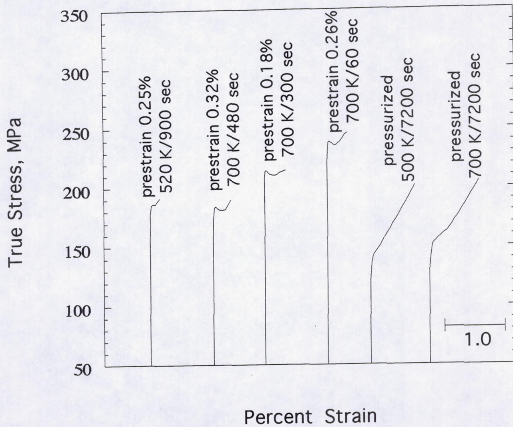
Figure 36. Room-temperature stress-strain curves illustrating the influence of various prestraining and annealing treatments on the tensile flow behavior of CP-NiAl.
