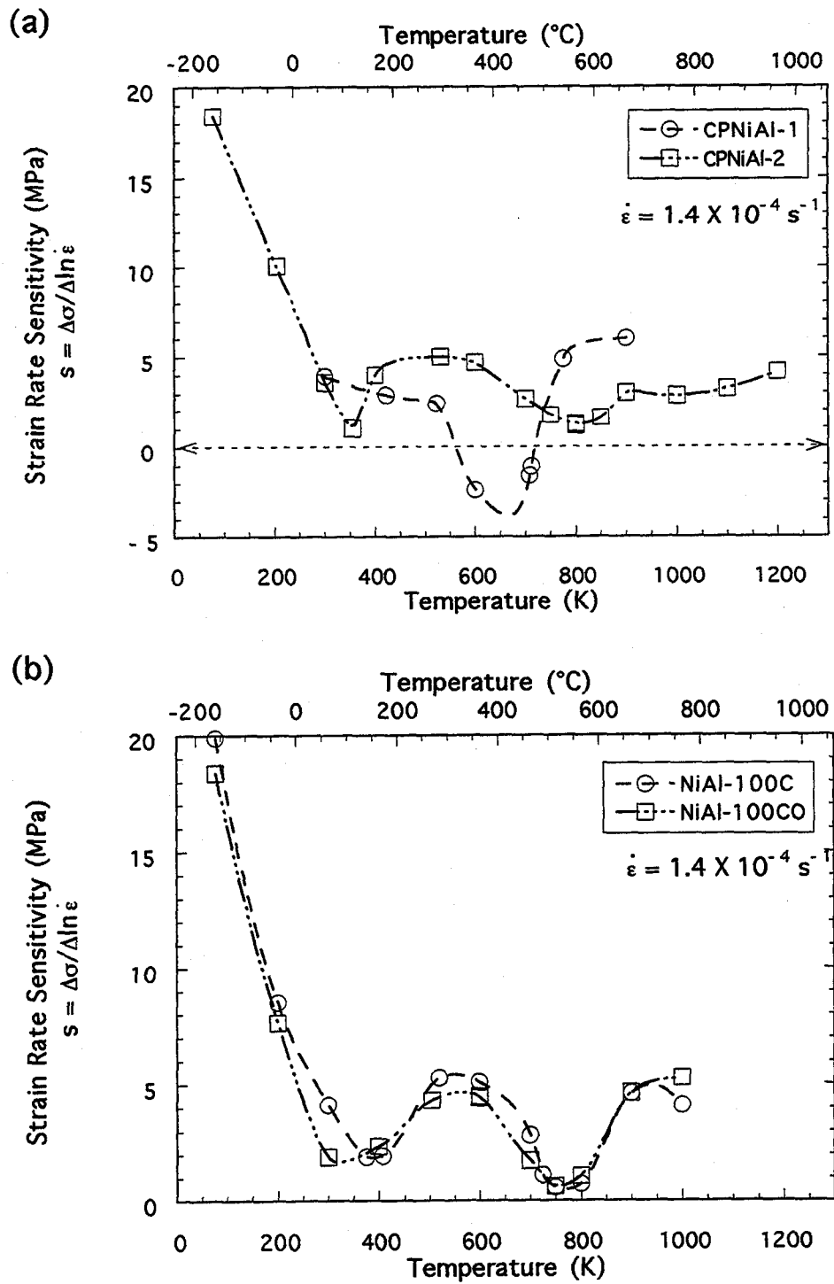
Figure 49. Temperature dependence of the SRS, s = \Delta\sigma/\Delta\ln \dot{\epsilon} : (a) CPNiAl-1 and CPNiAl-2; (b) NiAl-100C and NiAl-100CO; (c) NiAl-300C and NiAl-300CO; and (d) NiAl-N and NiAl-Ti.
