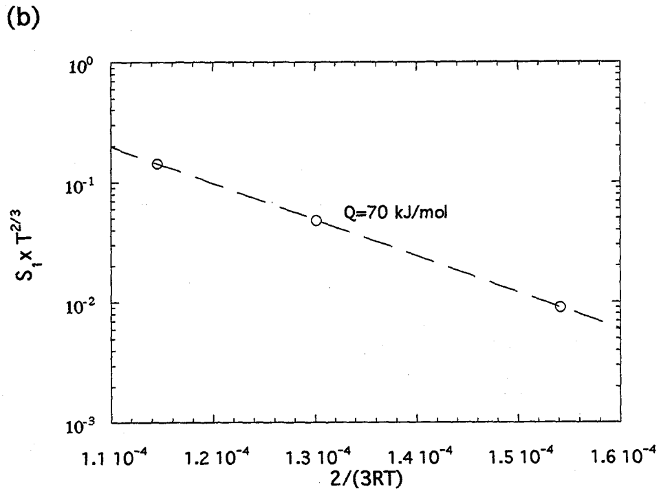
Figure 45. Demonstration of the Hartley method [38] for determination of the activation energy for yield point return. (a) Strain aging parameters versus t^{2/3} for CPNiAl-1 aged at 520, 616 and 700 K; (b) determination of the activation energy for yield point return using the Hartley method.
