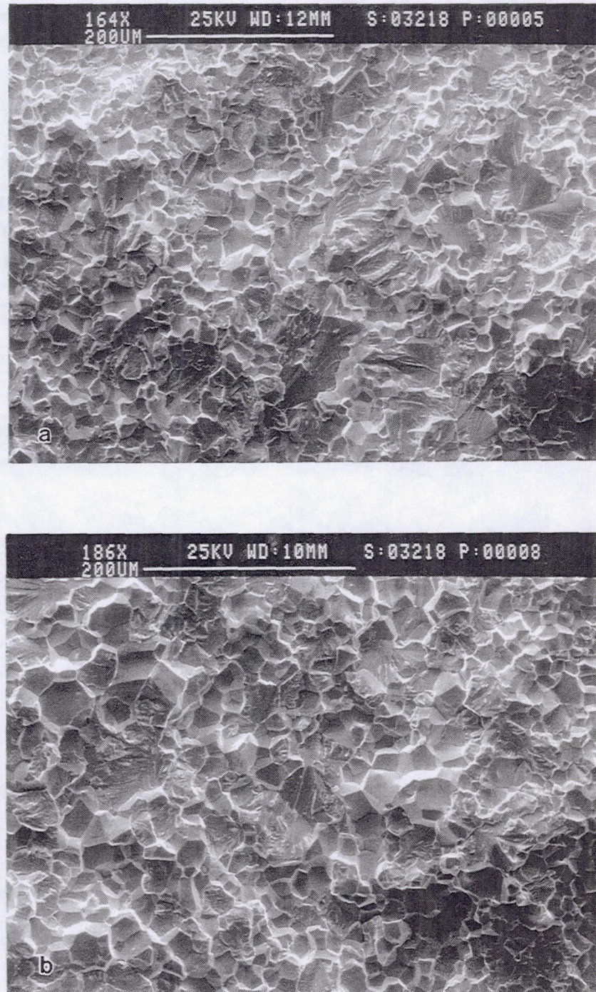
Figure 32. Fracture surfaces of NiAl-100C following tensile testing at room-temperature: (a) as-extruded and (b) after annealing at 1100 K for 2 h followed by furnace cooling.
