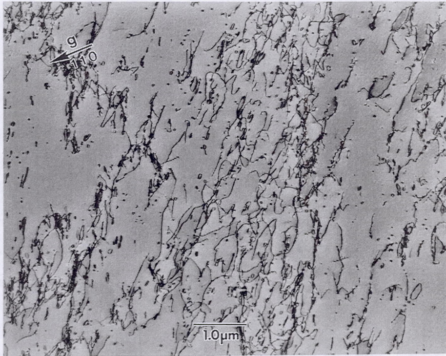
Figure 62. Dislocation morphology observed in CPNiAl-1 after 11% deformation at 1000 K.
