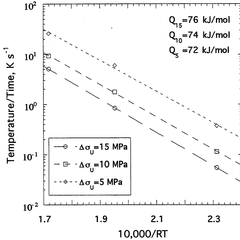
Figure 44. Arrhenius representation of the strain aging data for CPNiAl-1.
