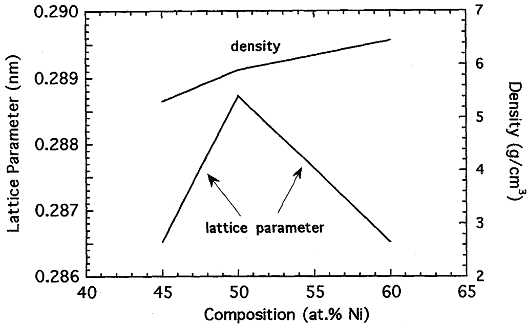
Figure 3. Variation in room-temperature lattice parameter and density of NiAl as a function of stoichiometry (Data compilation from [18]).
