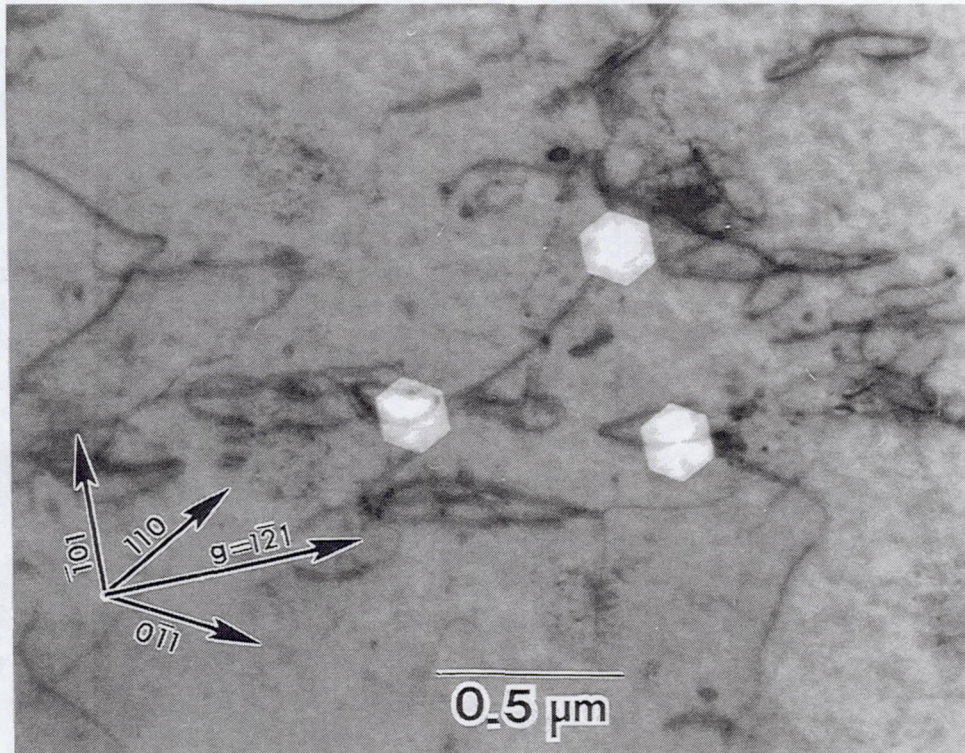
Figure 18. Faceted voids observed in HP-NiAl. Voids result from point defect agglomeration during the 1000 K/2 h/FC anneal.
