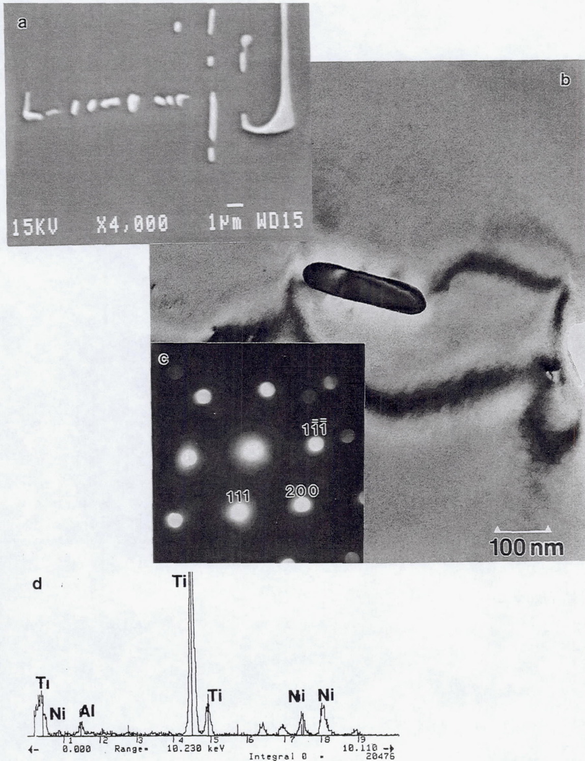
Figure 21. Stringers observed in NiAl-Ti: (a) Backscattered scanning electron micrograph of TiC stringers in NiAl-Ti; (b) BFTEM micrograph of a large TiC precipitate; (c) TEM microdiffraction pattern from the TiC precipitate ( [01\bar{1}] TiC zone axis); and (d) EDS spectra for the particle in (c) indicating the presence of Ti.
