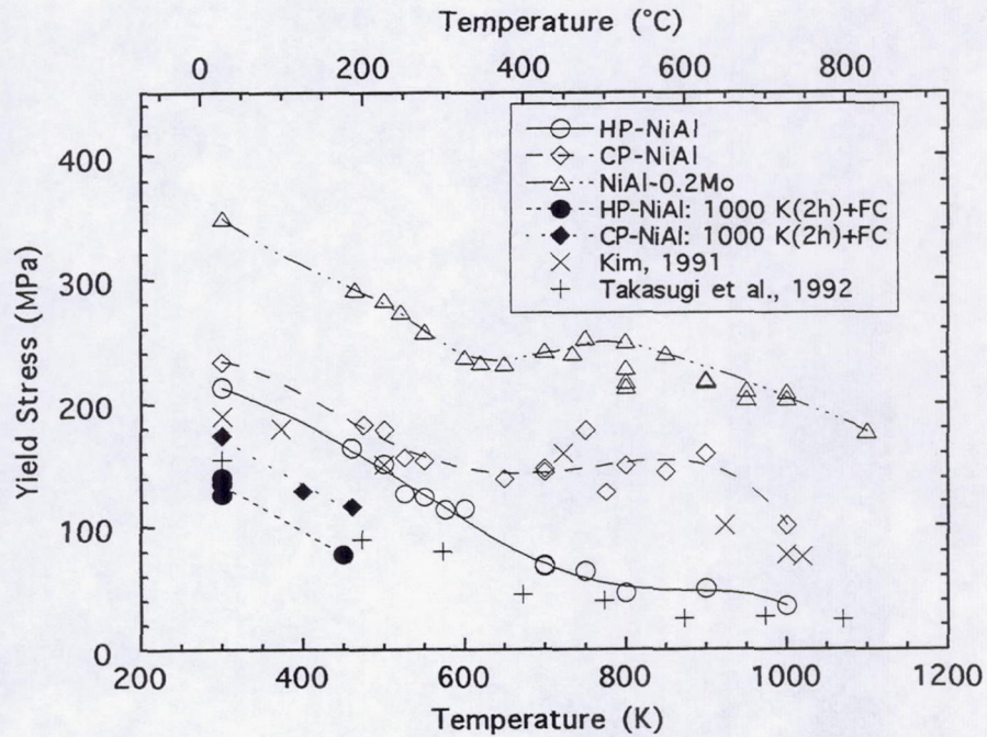
Figure 14. The temperature dependence of the 0.2% offset yield stress for HP-NiAl, CP-NiAl, and NiAl-0.2Mo single crystals and additional data from the literature.
