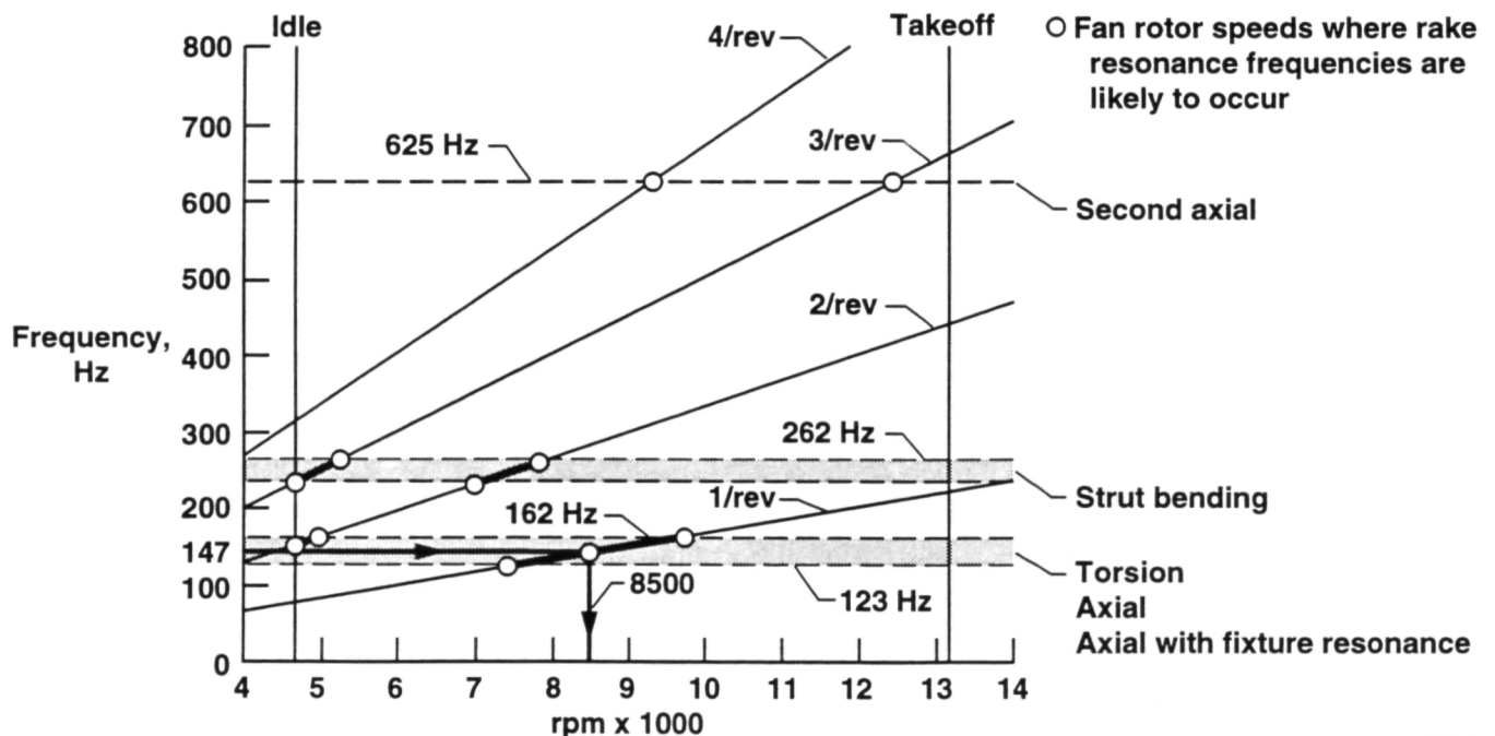
Figure 13. Campbell diagram showing rake vibration responses.
