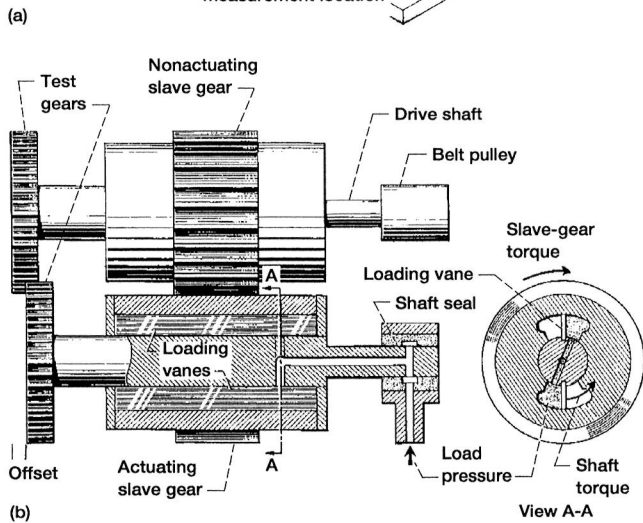
Figure 1.—NASA Lewis Research Center's gear fatigue test apparatus. (a) Cutaway view. (b) Schematic diagram.
