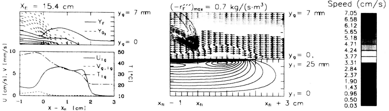
Fig. 7 Predicted velocity, fuel concentration, temperature, and flow field contours ( A = 5, E_g = 1, t = 5.0 s)
