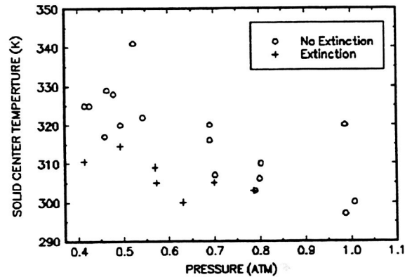
Figure 6 Solid Center Temperature vs. Pressure in Low-g (Lear Jet) with a Forced Flow of 10 cm/sec in air (subject to g-jitter)
