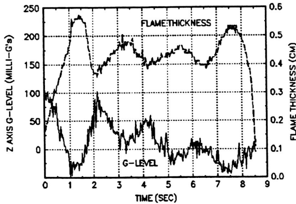
Figure 5 Flame Thickness & G-level vs. Time Pressure = 0.79 atm Solid Center Temperature = 303 K
