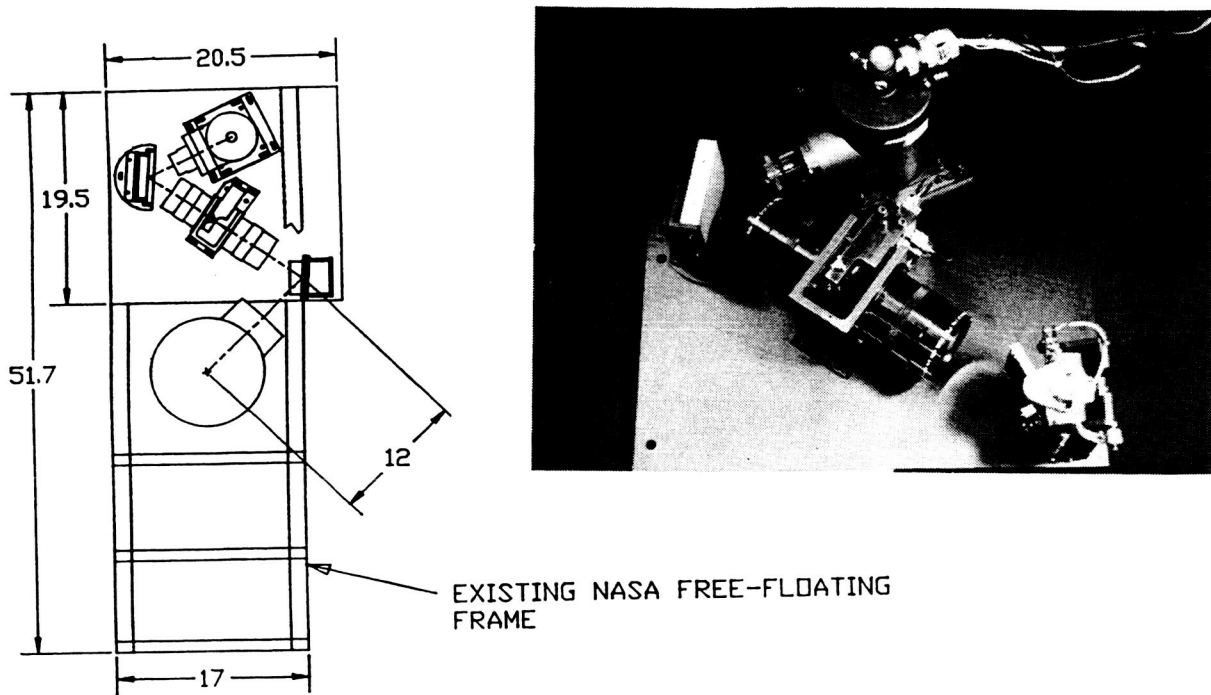
Figure 5. Optical Hardware and Overall Layout
