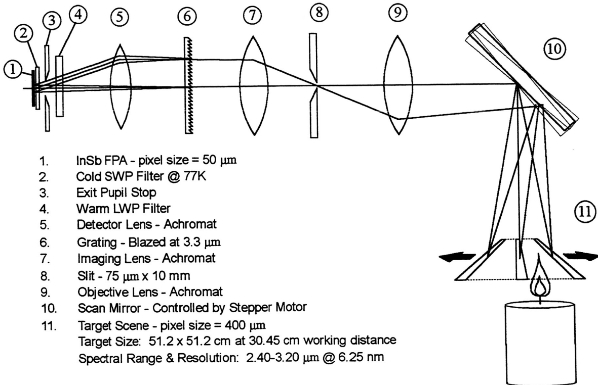
Figure 4. Optical Configuration
