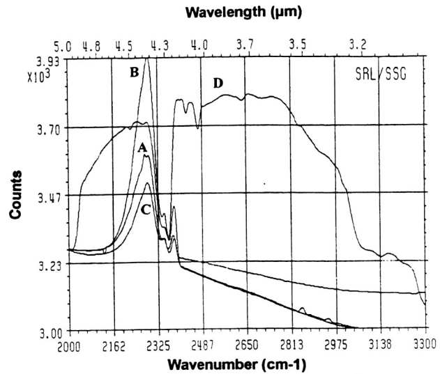
NASA Lewis Spectrometer Torch Data
