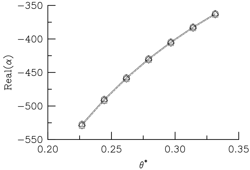
(a) Real part of \alpha .
