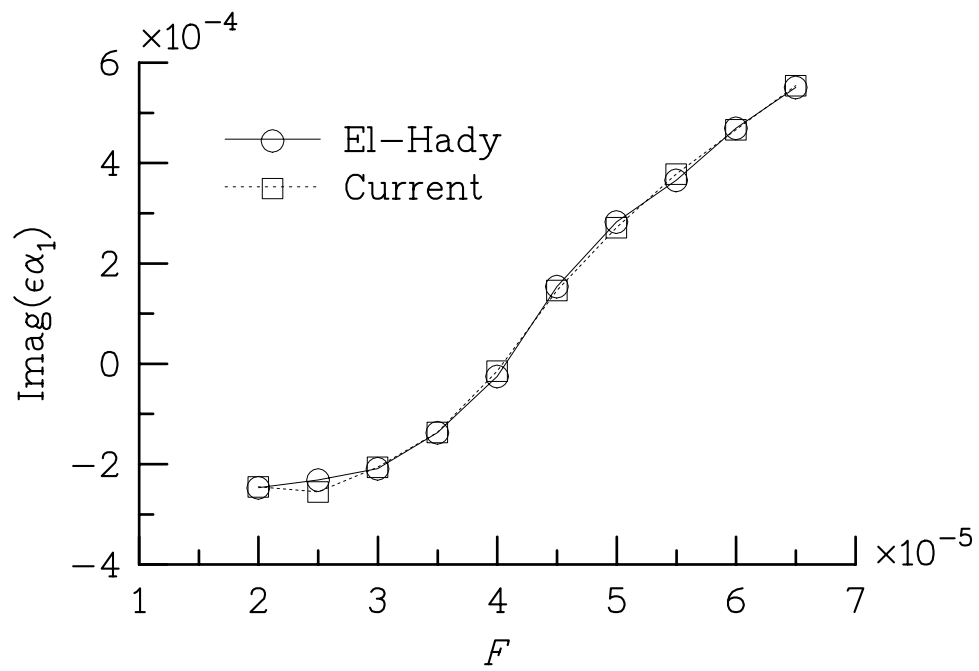
Figure 1. Nonparallel correction to growth rate at R = 1000 in a Blasius boundary layer: comparison with El-Hady [2].
