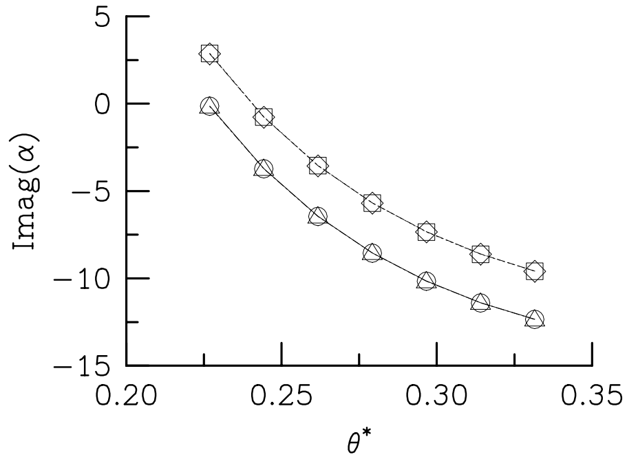
(b) Imaginary part of \alpha .
