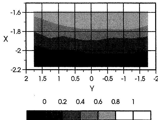
Figure 7: Spanwise Variation of Intermittency in the Undisturbed Interaction
