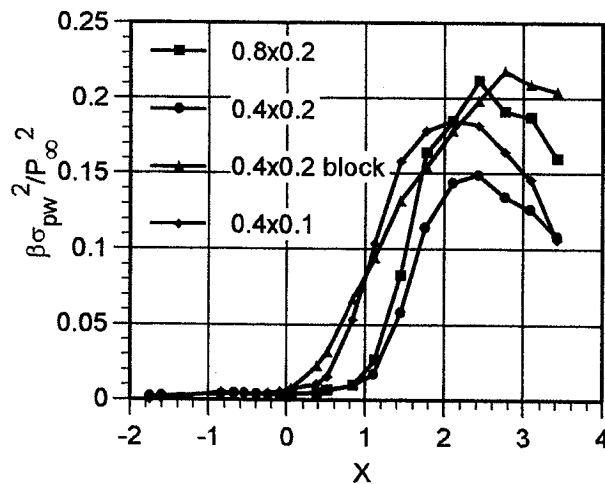
Figure 18: Wall Pressure Variance Distributions with BLSs Upstream and L=0.95
